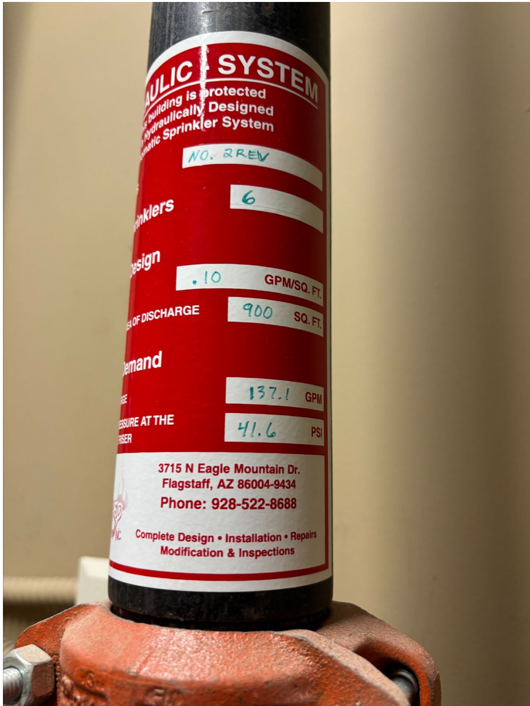
PICTURE 5 Special Service Building Riser (Two Story Building)
