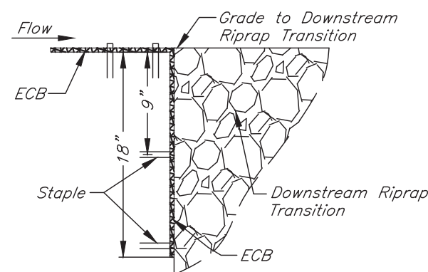
DOWNSTREAM END DETAIL SECTION
