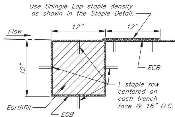
UPSTREAM START DETAIL SECTION
