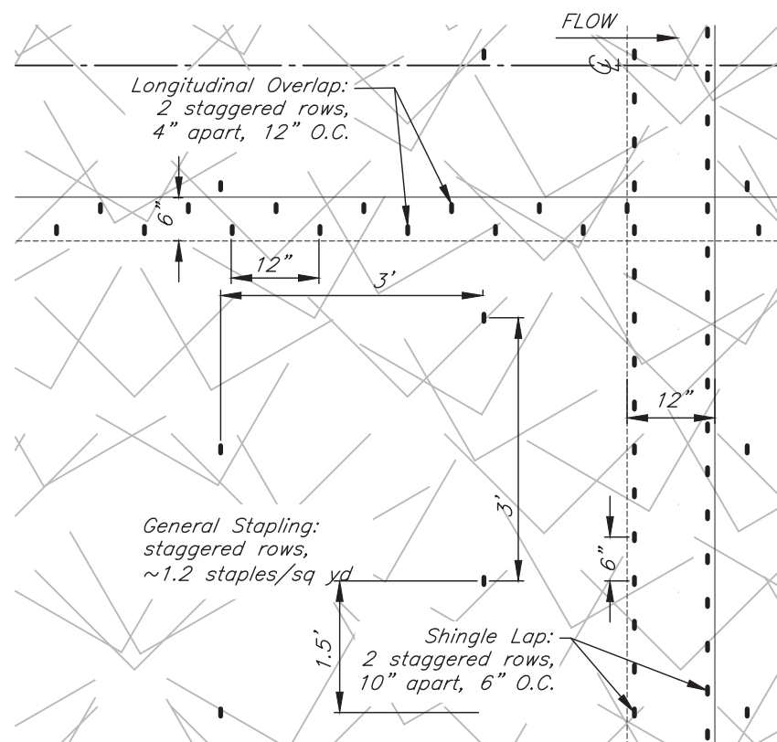
STAPLE DETAIL PLAN
