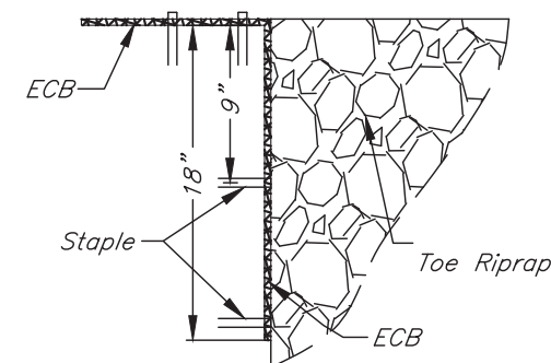
TOE RIPRAP DETAIL SECTION
