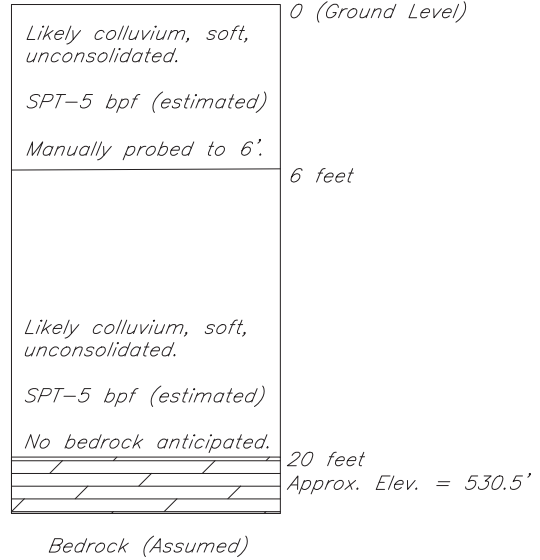
Soil Investigation #1 & #2 Log Not to Scale
