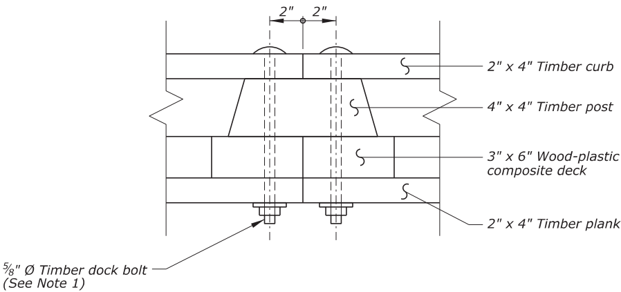
DISCONTINUOUS CONNECTION
