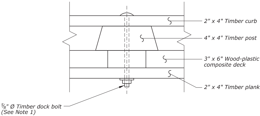
CONTINUOUS CONNECTION
