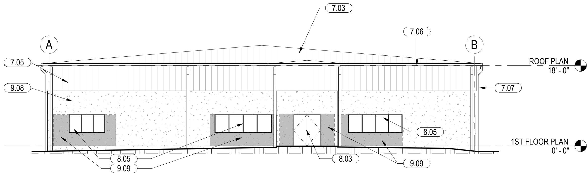
4 WEST ELEVATION SCALE: 3/32" = 1'-0"
