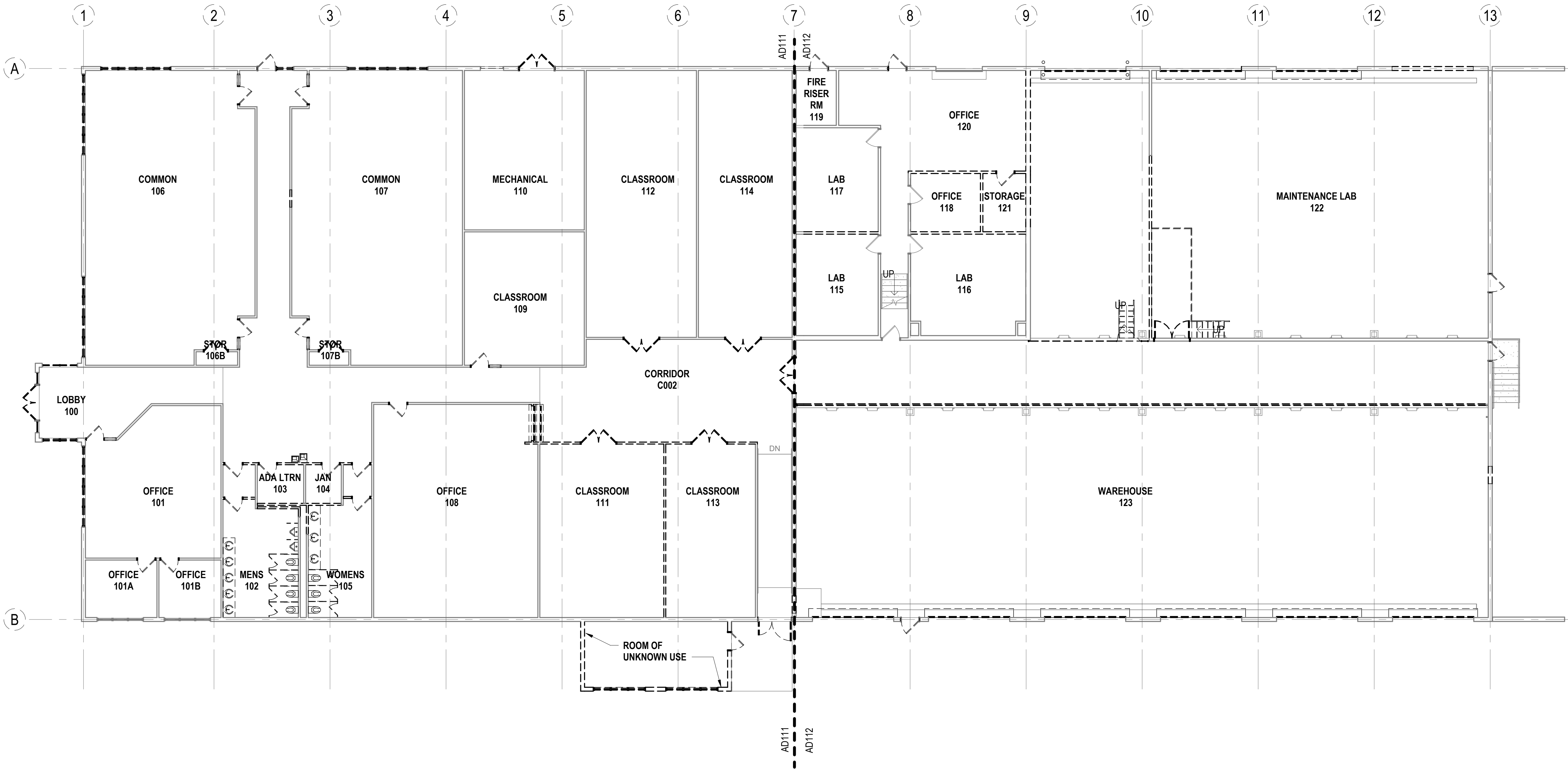
1 COMPREHENSIVE - PRELIMINARY DEMOLITION PLAN SCALE: 1" = 10'-0"
