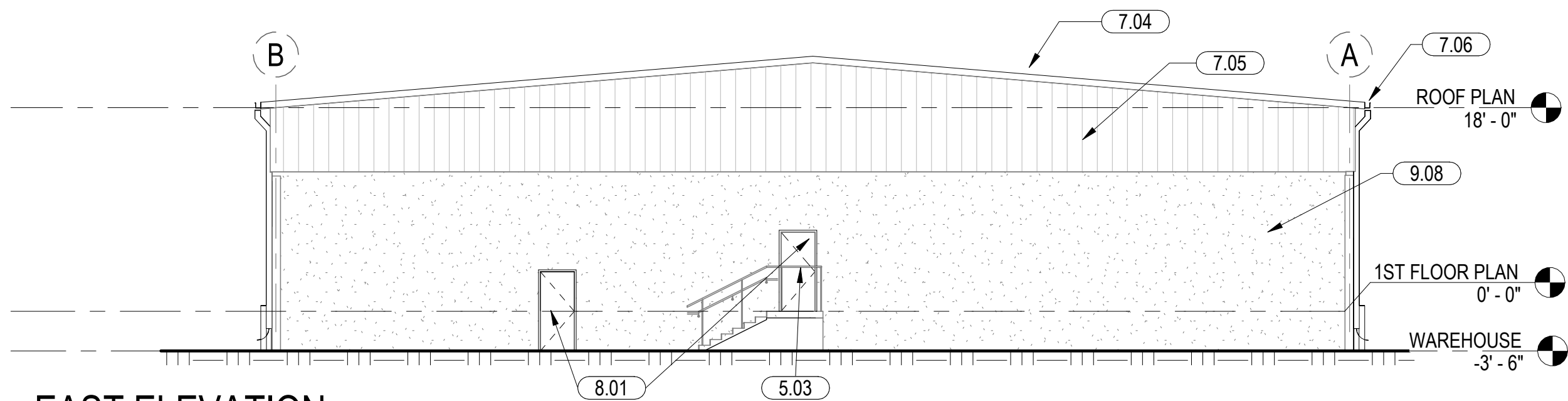
3 EAST ELEVATION SCALE: 3/32" = 1'-0"
