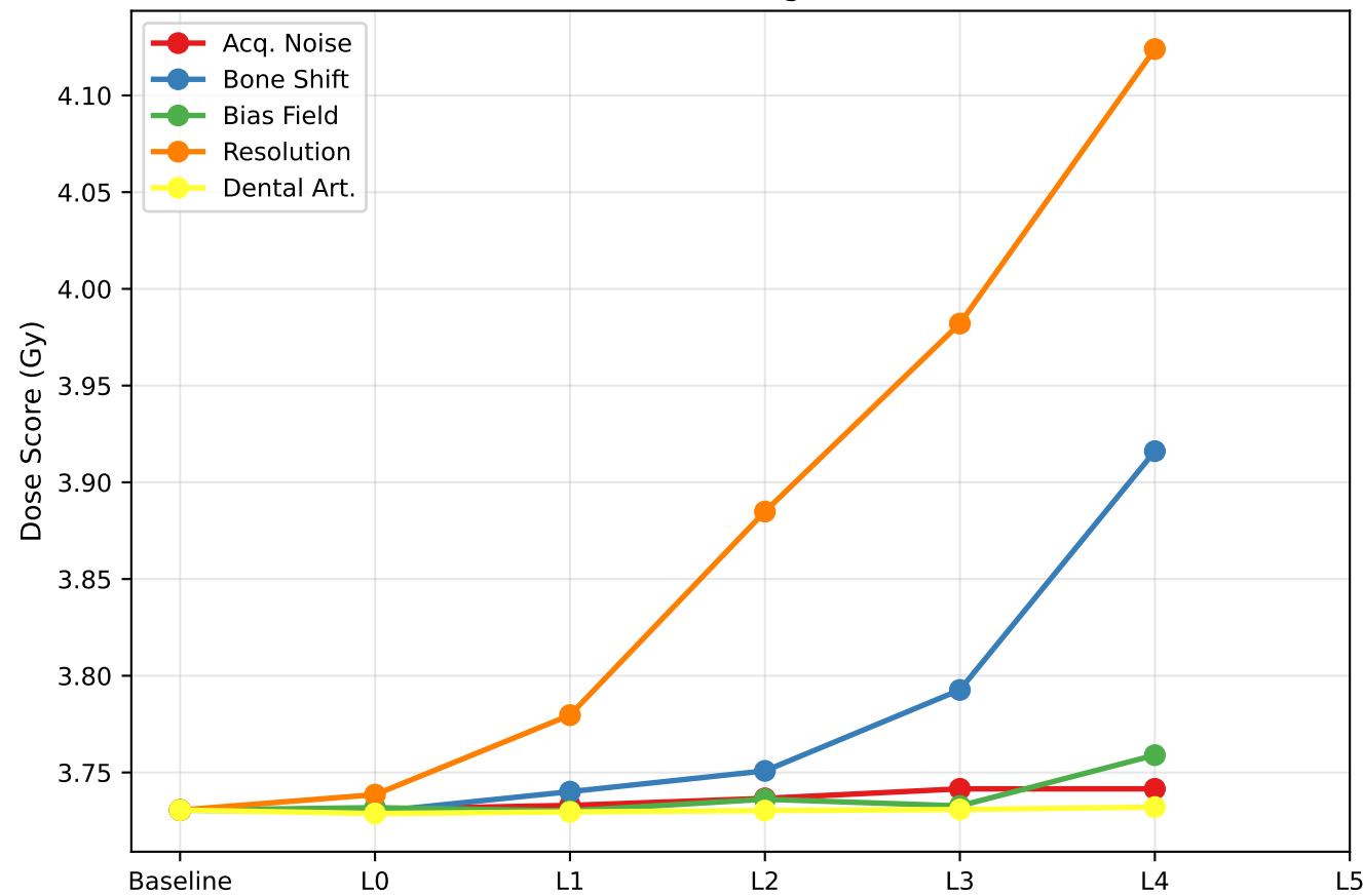
Dose Score Degradation
