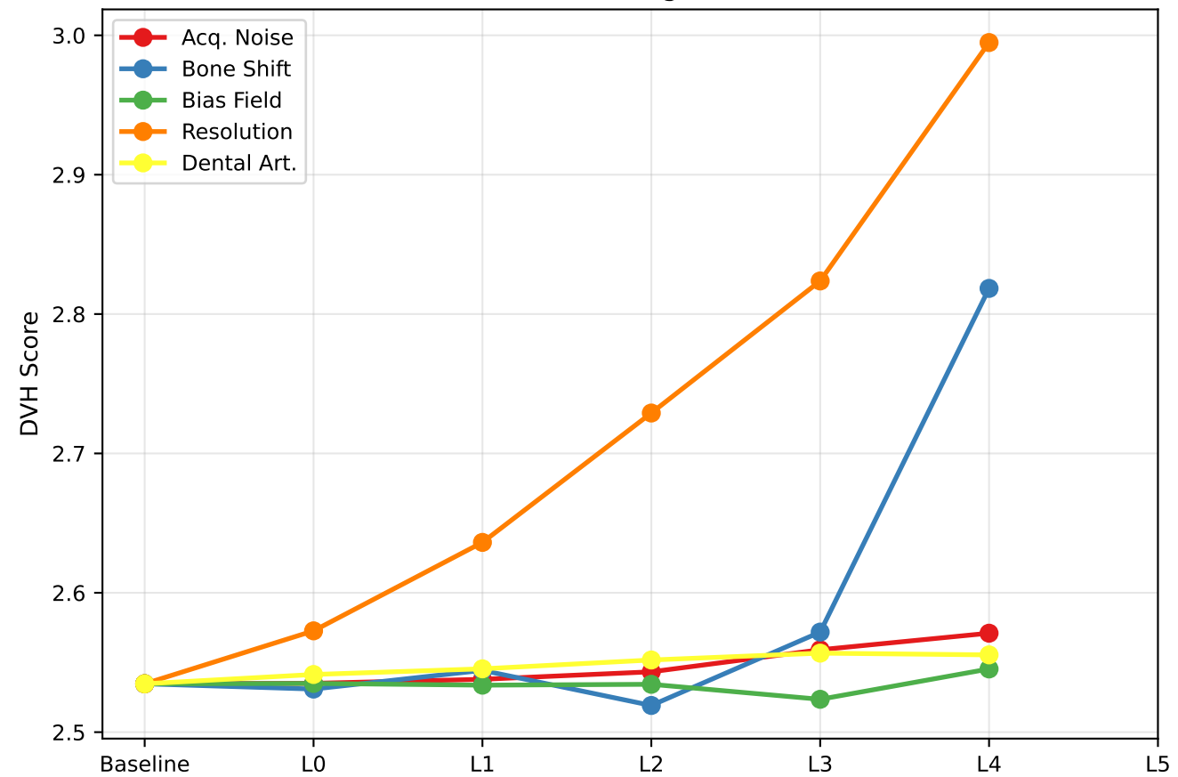
DVH Score Degradation
