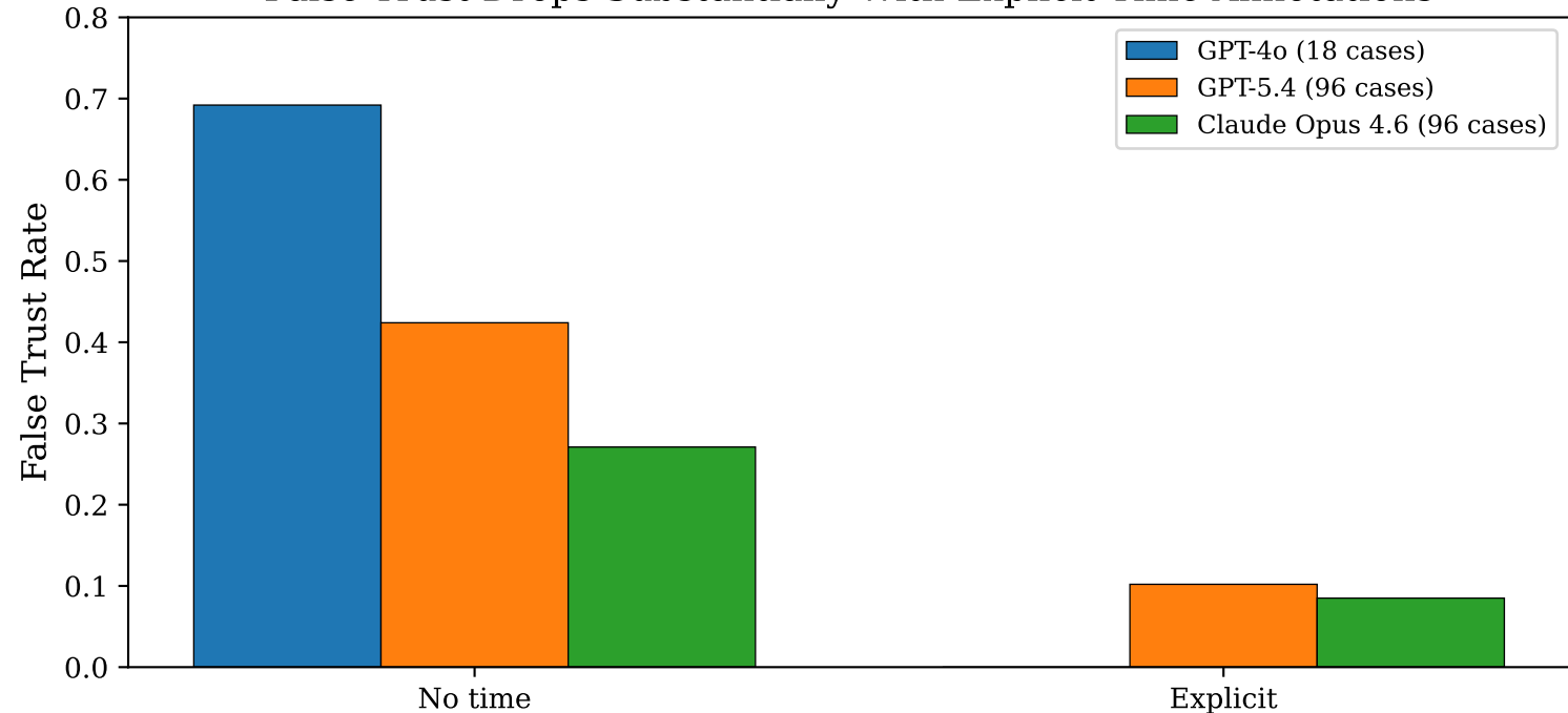
False Trust Drops Substantially With Explicit Time Annotations
