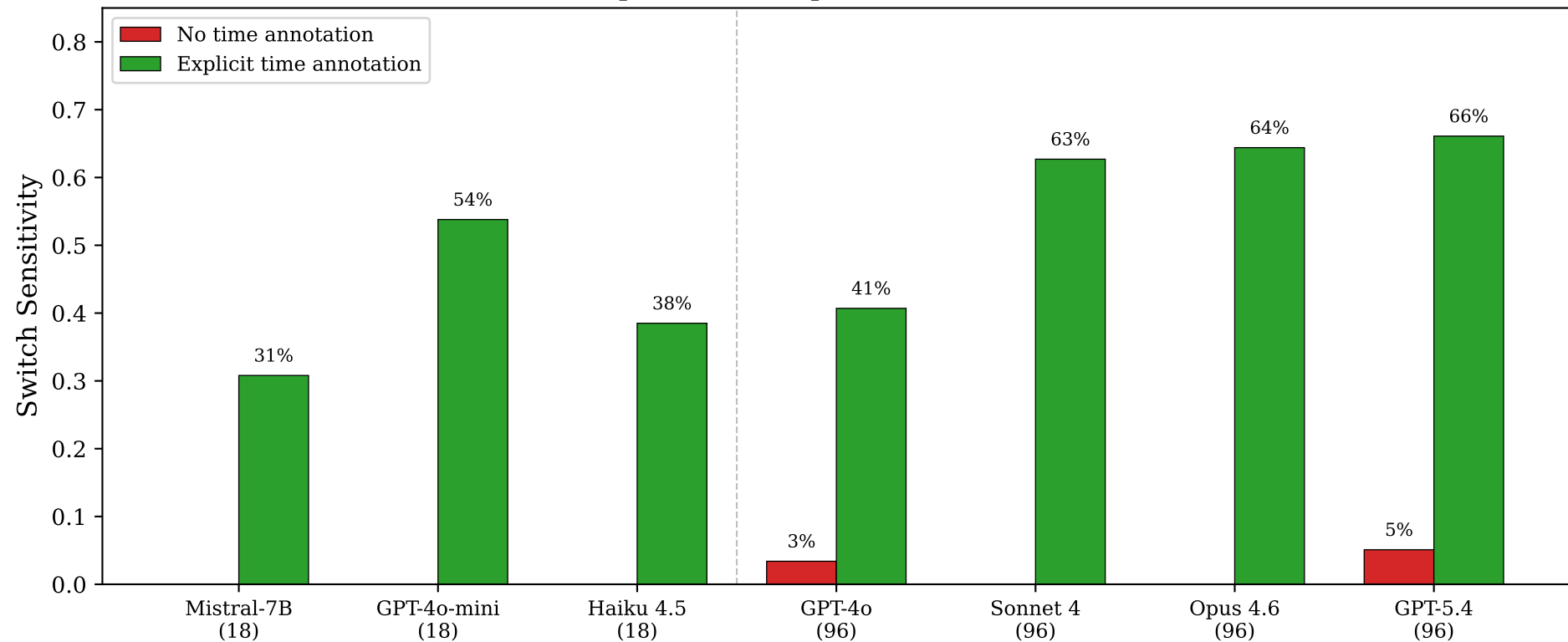
The Temporal Blind Spot Across Seven Models
