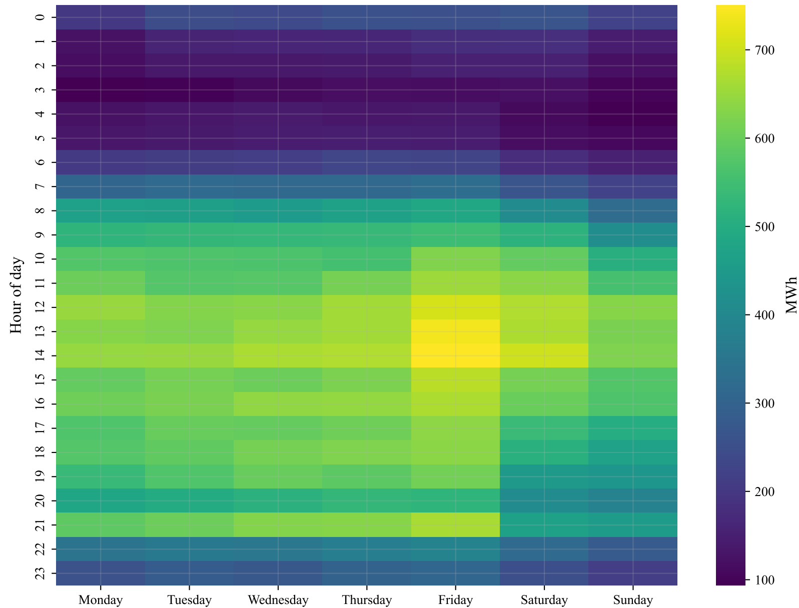
Grid demand heatmap: DCFC charging energy by hour and weekday
