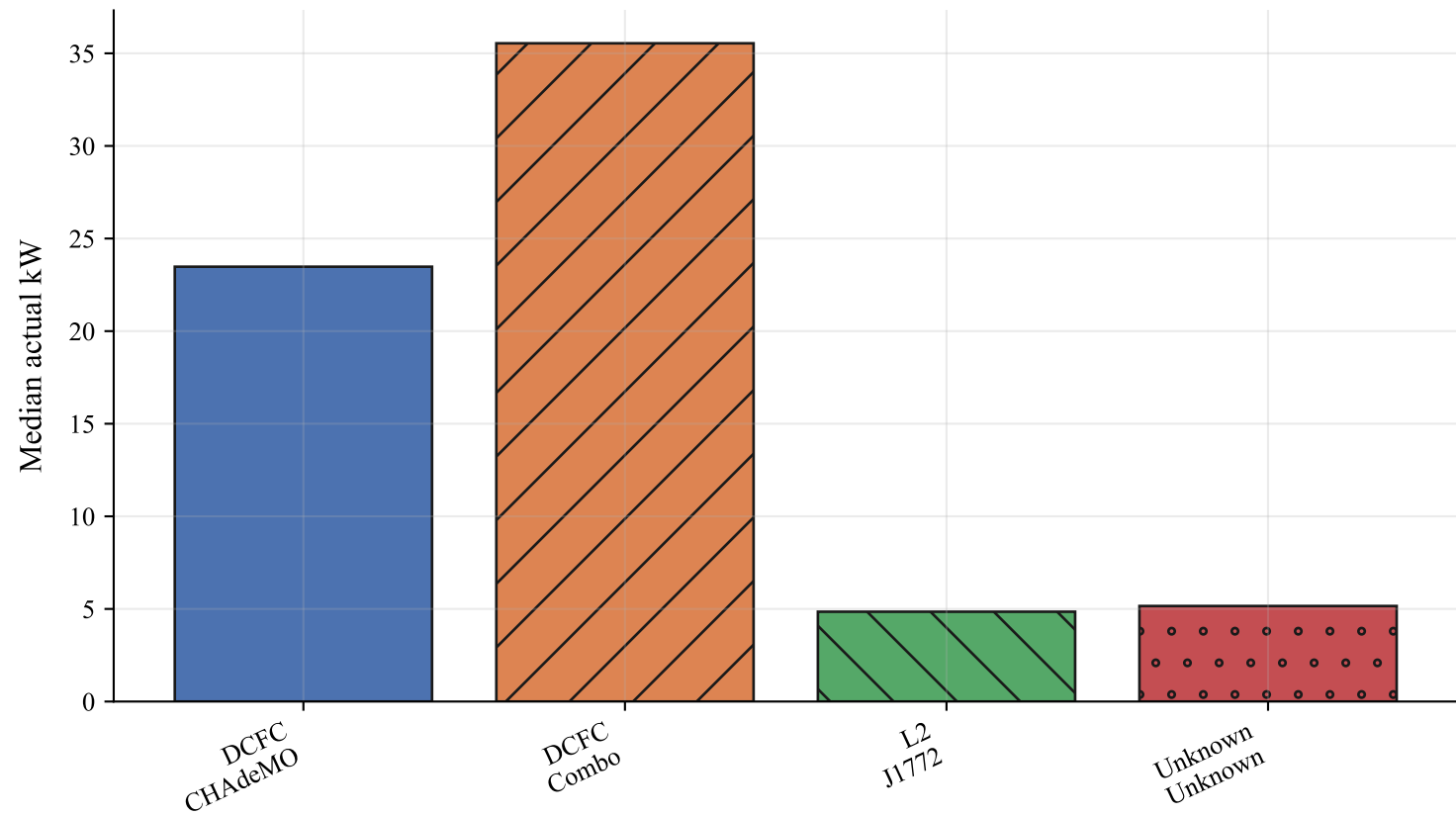
Actual charging rate by level and connector
