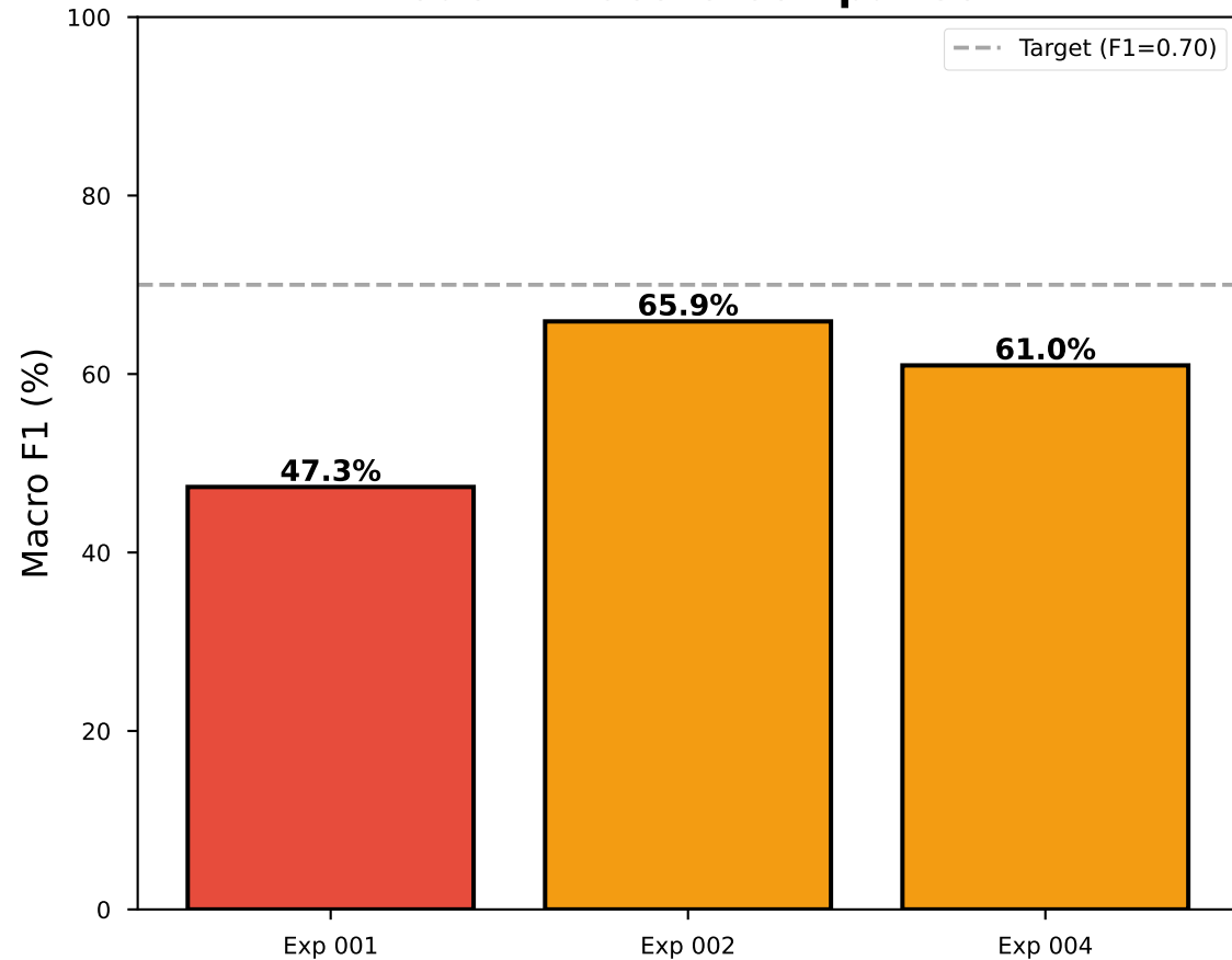
Model F1-Score Comparison
