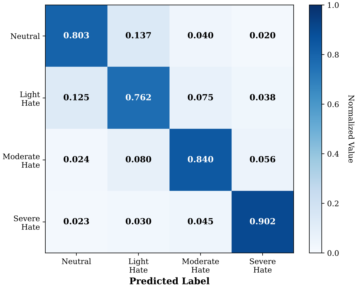
Confusion Matrix (Normalized) IndoBERT + Label Smoothing (epsilon=0.1)
