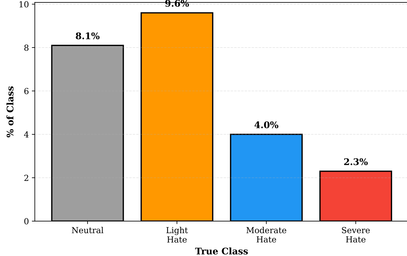
Hard Negatives as Percentage of Each Class
