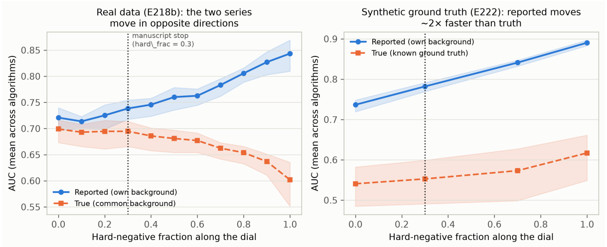
Figure 4: The selection criterion on a design’s own background (solid) keeps rising to the edge of the dial; the true performance (dashed) does not, so the criterion has no interior optimum. Left: real data — the two series move in opposite directions. Right: synthetic ground truth — reported performance moves about twice as fast as truth. The dotted vertical line marks the manuscript’s stop at hard_frac = 0.30; the dial ends at 1.0.
