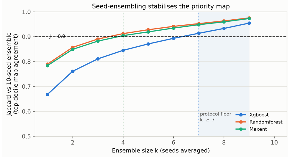
Figure 6: Agreement of an ensemble of k seeds with the full 10-seed ensemble on the top-decile priority map, one line per learner. A single seed agrees at Jaccard \approx 0.65 – 0.80 ; k^* = 4 – 7 suffices for Jaccard \geq 0.90 , and k \geq 7 is the protocol floor (shaded).
