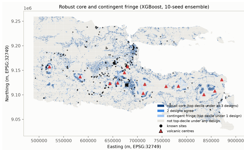
Figure 5: Robust core and contingent fringe for XGBoost under a 10-seed ensemble, cells coloured by how many of the three background designs placed them in the top decile. The core concentrates on the accessible lowlands that hold the known record; the contingent fringe is the remote upland on which background assumptions disagree (median 1.0 km from roads and 1,107 m elevation in the MaxEnt fringe).
