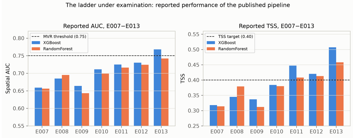
Figure 2: Reported AUC and TSS across the seven experiments of the published pipeline (E007–E013; Table 3). This is the ladder under examination; §3.2 asks whether the rise between E007 and E013 is real.
