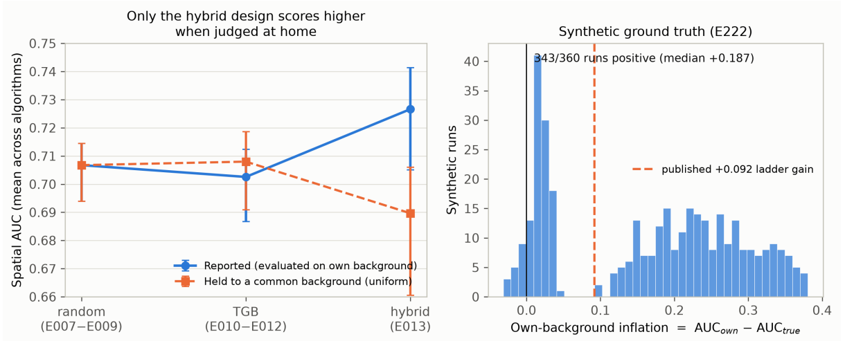
Figure 3: The evaluation artefact. Left: reported AUC (evaluated on a design’s own background) against the same designs held to a common background (uniform). Only the hybrid design scores higher when judged at home. Right: own-background inflation across 360 synthetic runs of known ground truth (343/360 positive, median +0.187 ); the published +0.092 ladder gain is marked.
