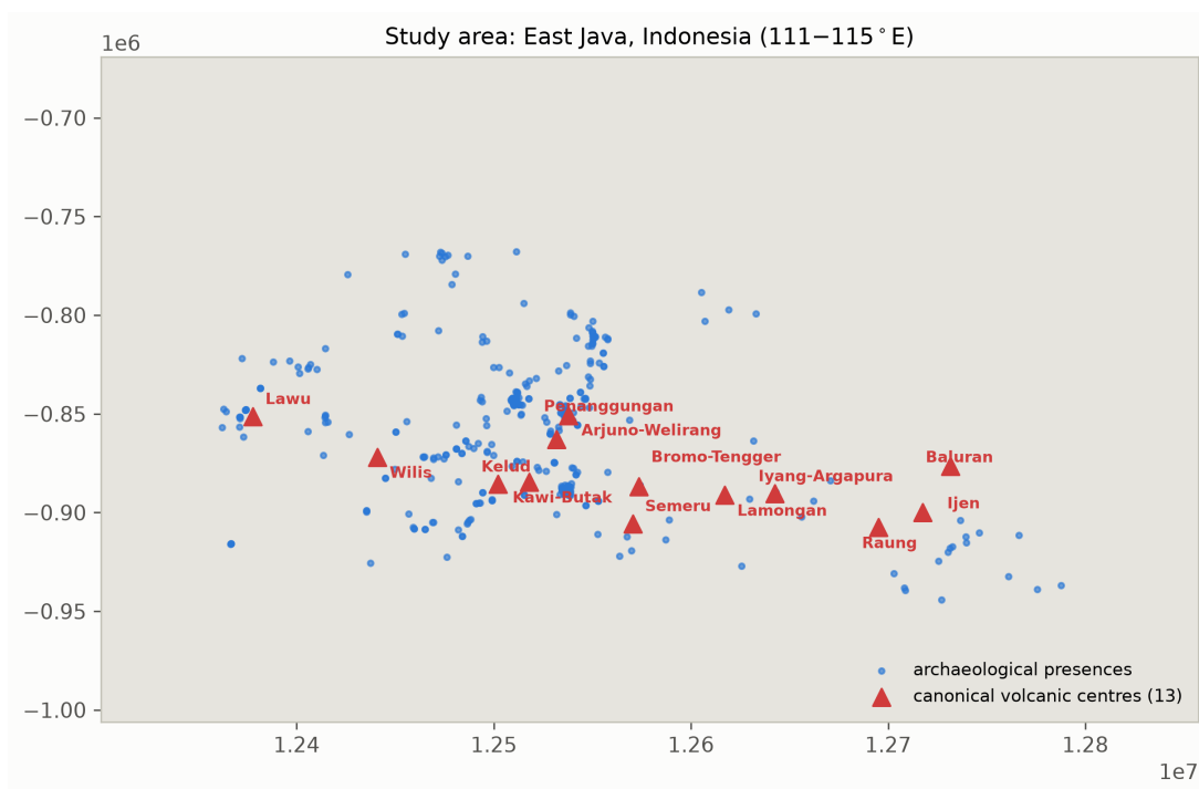
Figure 1: Study area in East Java, Indonesia, showing the presences used for modelling and the 13 canonical volcanic centres inside the paper’s stated bounds (111–115°E), used as post-hoc diagnostics only.
