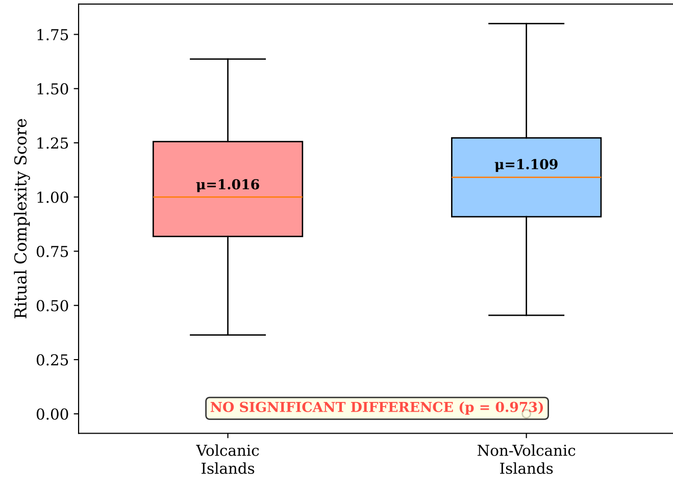
E039a: Volcanic vs Non-Volcanic Islands Mann-Whitney p = 0.973
