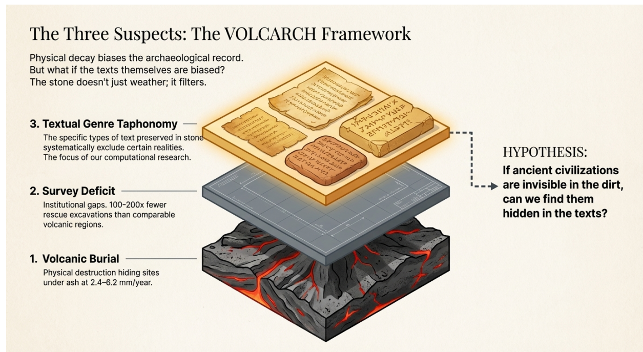
Figure 1: The three layers of taphonomic bias addressed in this paper. Layer 1 (bottom): volcanic burial physically conceals sites at 2.4–6.2 mm/year. Layer 2 (middle): institutional survey deficit—Indonesia conducts 100–200× fewer rescue excavations than comparable volcanic regions. Layer 3 (top): textual genre taphonomy—the types of text preserved in stone systematically exclude physical geography. This paper focuses on Layer 3, asking: if civilizations are invisible in the dirt, can we find them hidden in the texts?
