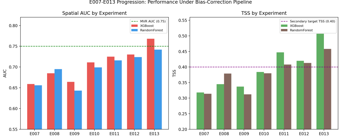
Figure 2: AUC/TSS progression E007–E013. [FIGURE: under block E, overlay the common-evaluation-background values so the artefact is visible against the ladder in one panel.]
