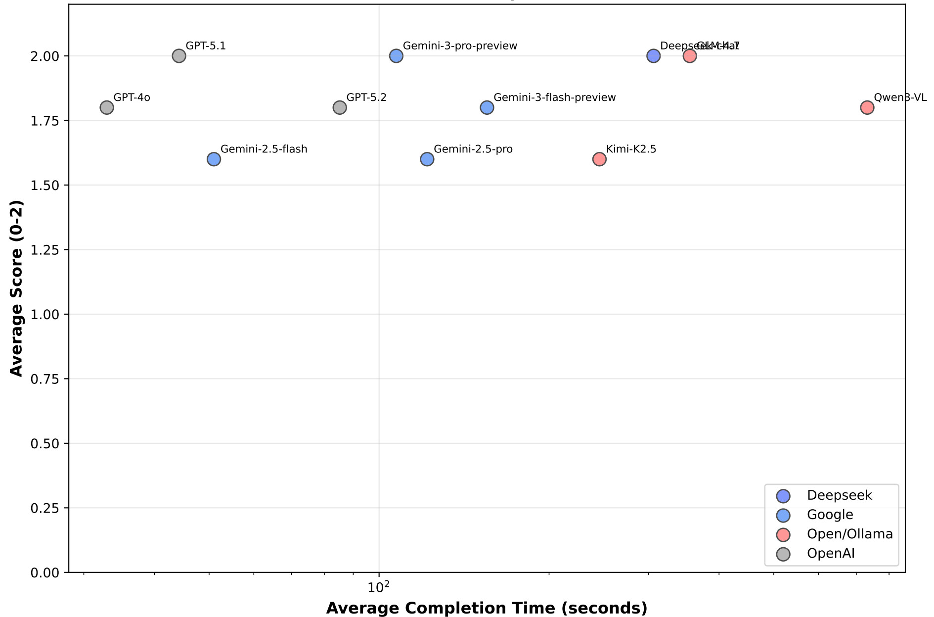
Time vs Quality Tradeoff
