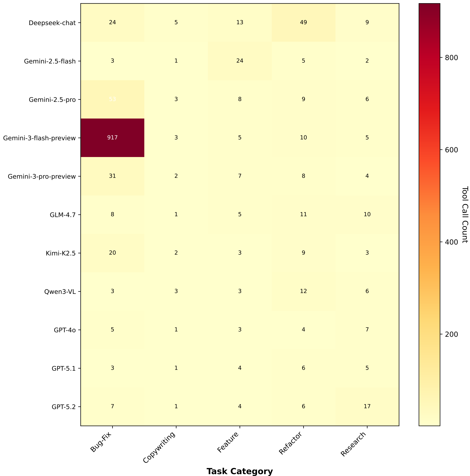
Tool Usage Heatmap by Model and Task
