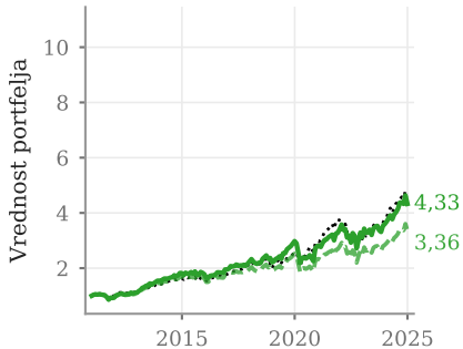
MASTER + SO
