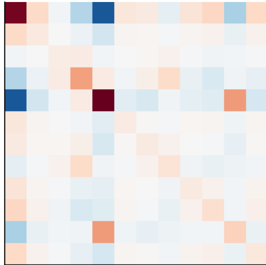
\Sigma = BB^T + \text{diag}(\psi)
