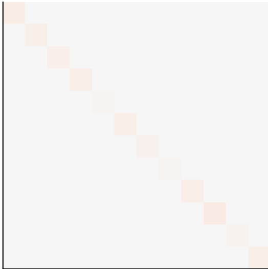
\text{diag}(\psi)
