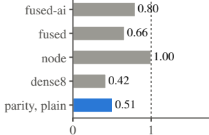
A100, FP32
