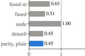
RTX 4090, FP32
