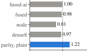
RTX 4090, FP32
