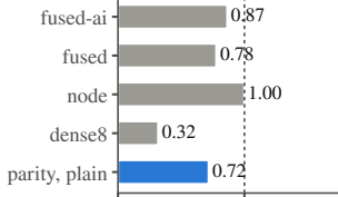
A100, FP32
