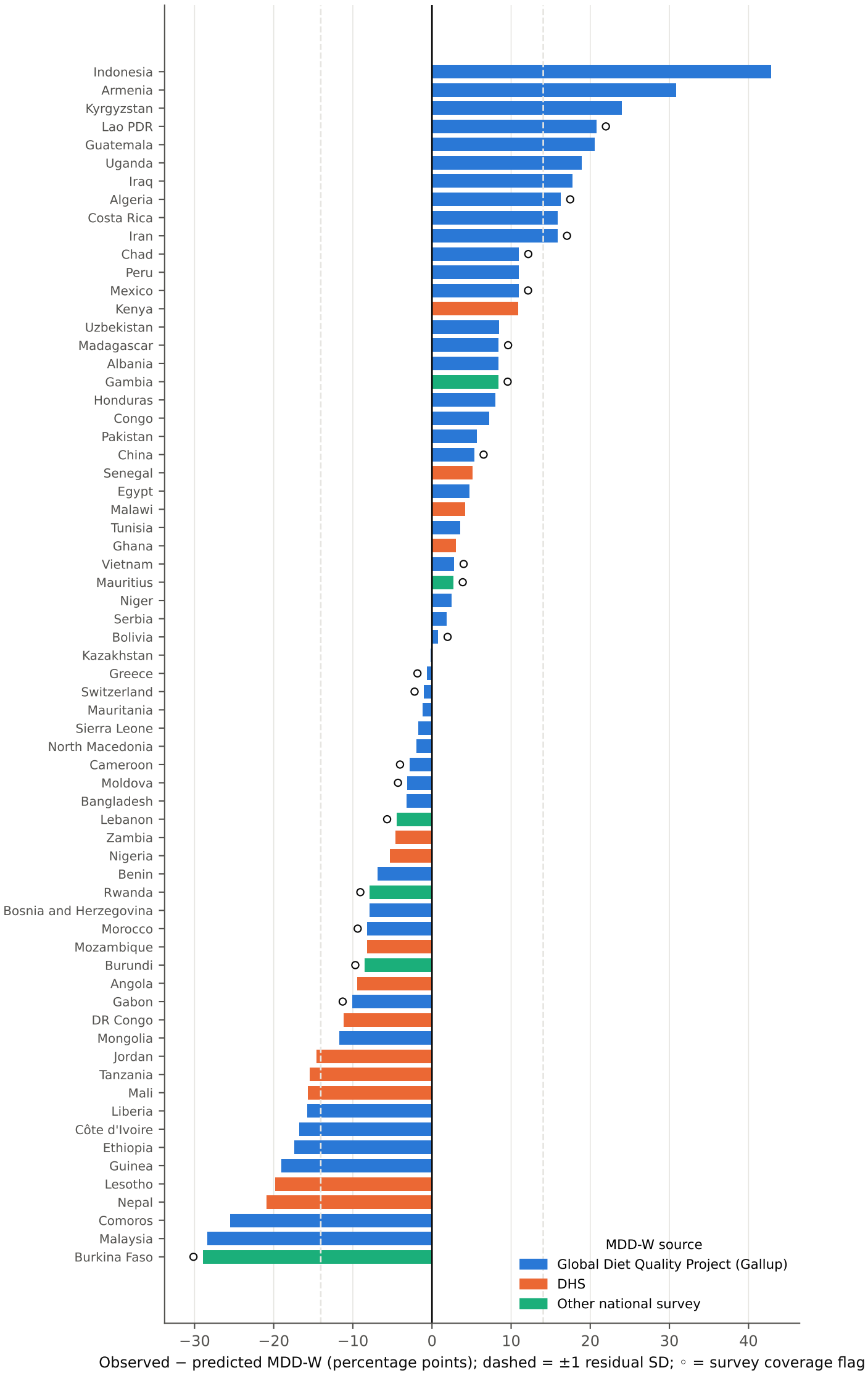
MDD-W relative to the level predicted by healthy-diet unaffordability
