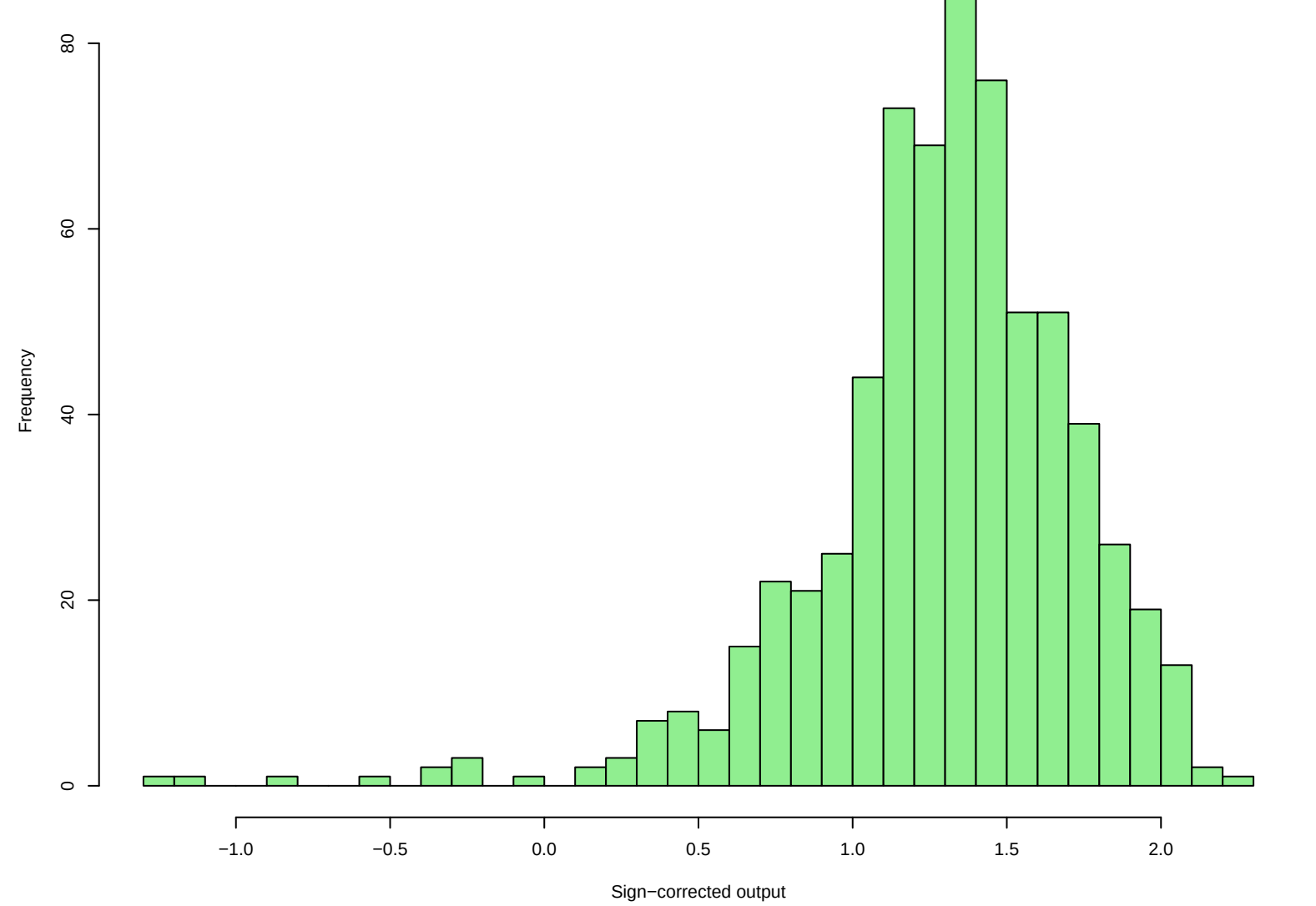
Rational quadratic kernel
