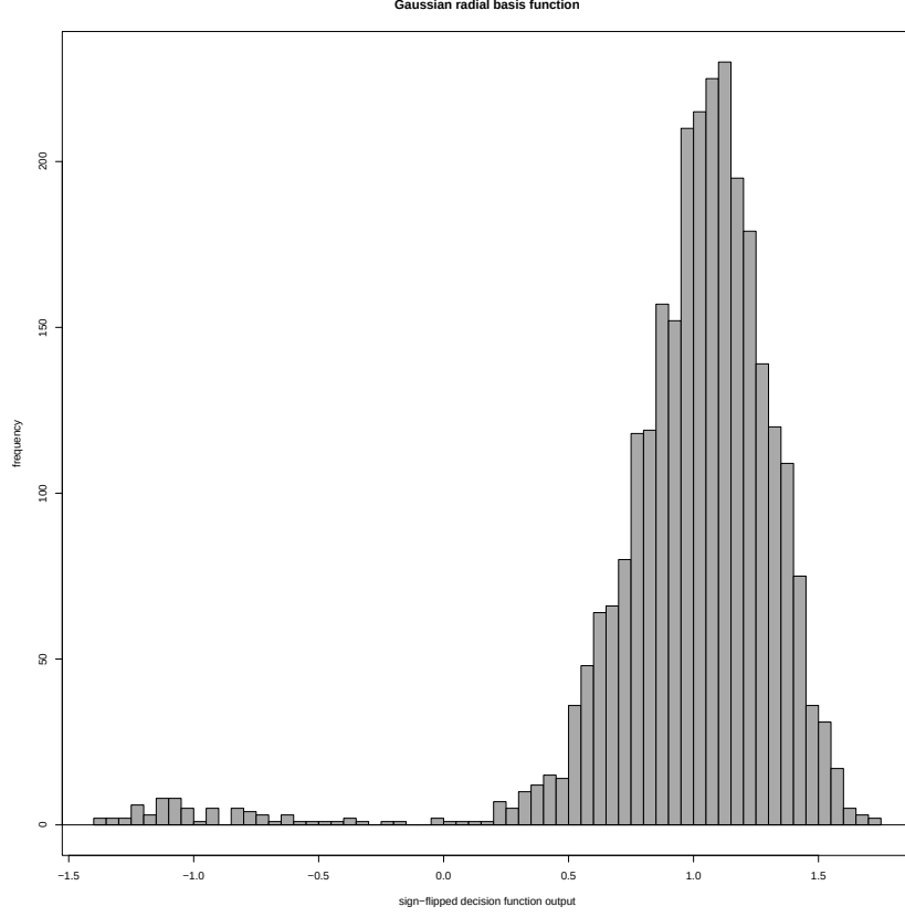
Figure 1: Count with respect to sign-corrected certainty degree.
