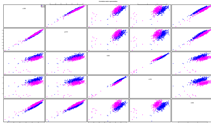
Figure 4: Scatterplots of sign-corrected certainty degree for every kernel vs every other one – c.006 is Cauchy kernel, g.013 Gaussian, l.006 Linear, s.021 Sigmoid, and t.006 Tanimoto; mouse datapoints are pink and human ones blue; concentration ellipses are drawn for each tag in concentration levels 0.5 and 0.9.
