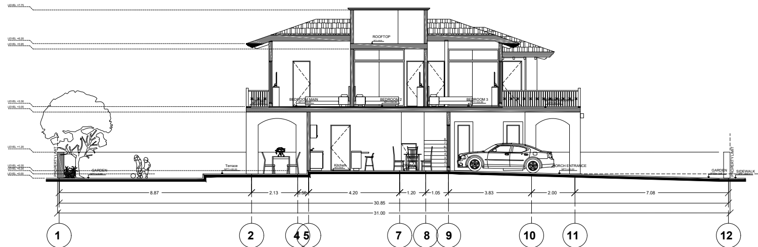
Corte A CASA COLONIAL JAZMIN SCALE 1:75
