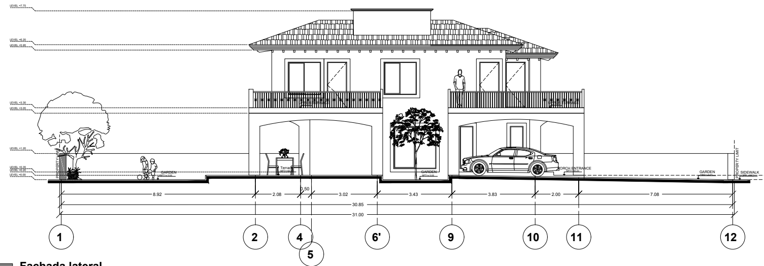
Fachada lateral CASA COLONIAL JAZMIN SCALE 1:75
