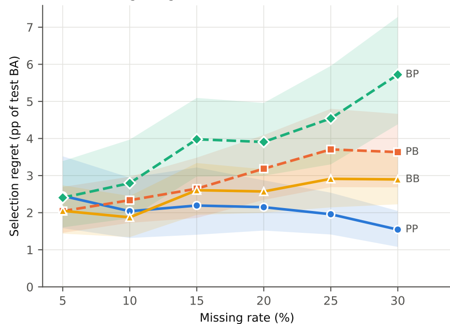
—●— PP (matched) - -■- - PB (mismatched) - -◇- - BP (mismatched) —▲— BB (matched) A Regret against the candidate-set test oracle
