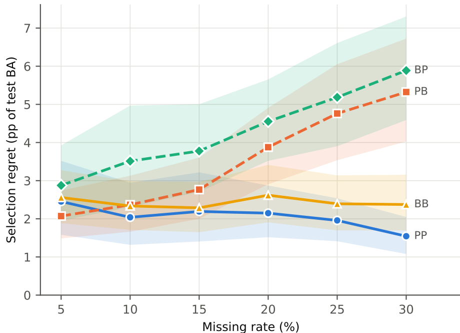
—●— PP (matched) -■- PB (mismatched) -◆- BP (mismatched) —▲— BB (matched) A Regret against the candidate-set test oracle
