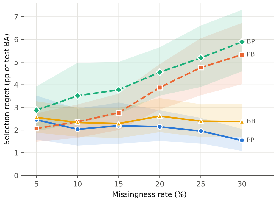
PP (matched) PB (mismatched) A Regret against the candidate-set test oracle
