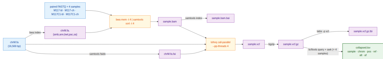
Figure 1. Data flow of the simplified mtDNA variant-calling workflow used in this study. Per-sample steps (alignment through tabix ) run independently for each of the four samples; the only inter-sample dependency is the final bcftools query + awk fan-in that builds collapsed.tsv .
