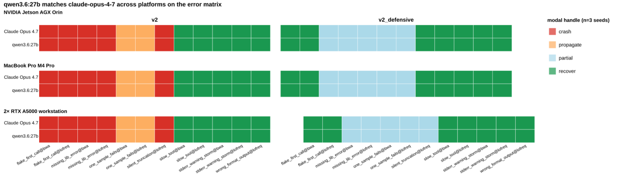
Figure 2: Figure 3. Per-cell error-handling outcome (recover / partial / propagate / crash) for claude-opus-4-7 and qwen3.6:27b across the 12-cell PATH-shim error matrix on three hardware platforms. Left column = v2 baseline plan; right column = v2_defensive plan. Rows within each panel are the two models. Cells are color-coded by the modal m_handle outcome across three seeds.
