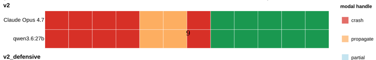
qwen3.6:27b matches claude-opus-4-7 cell-for-cell on the error matrix (modal handle across 3 seeds — identical on Jetson, MacBook Pro M4 Pro, and 2× RTX A5000)
