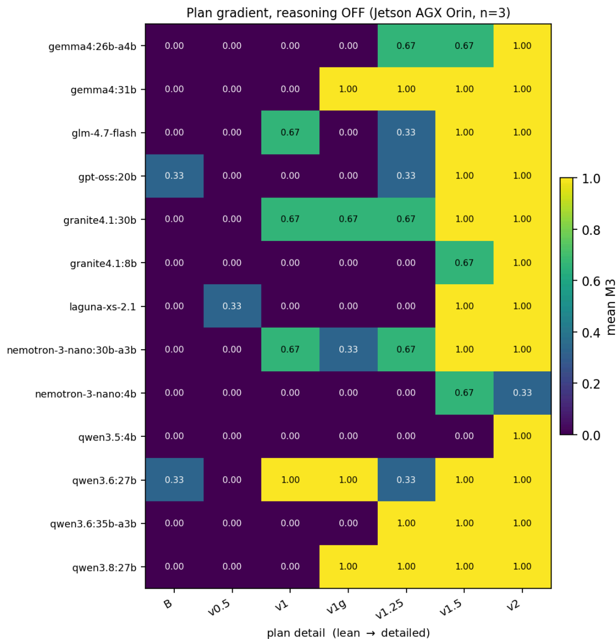
Figure 2. Plan gradient with reasoning disabled, Jetson AGX Orin, n = 3 seeds per cell. Rows are the twelve benchmark-1 local executors plus the out-of-sample addition qwen3.8:27b , thirteen rows in all. The twelve-model gradient totals given in the text exclude qwen3.8:27b , which was run separately and is shown here for comparison. Columns run left to right from no plan (Track B) to the most detailed plan (v2). Cell values are the mean tolerant Jaccard score (M3), which on this arm takes only the values 0 and 1 per run.
