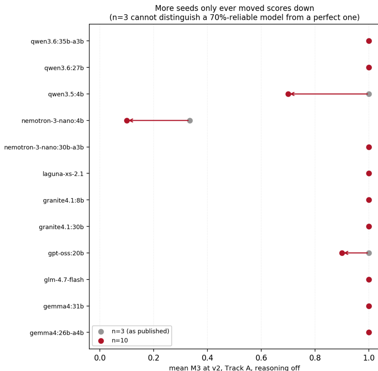
Figure 3. Repeated sampling at the headline condition (plan v2, Track A, reasoning off). Grey points are the n = 3 means as originally published; red points are the pooled n = 10 means. Every model that moved, moved down; no model rose. This is repeated sampling from one configuration, not independent replication.
