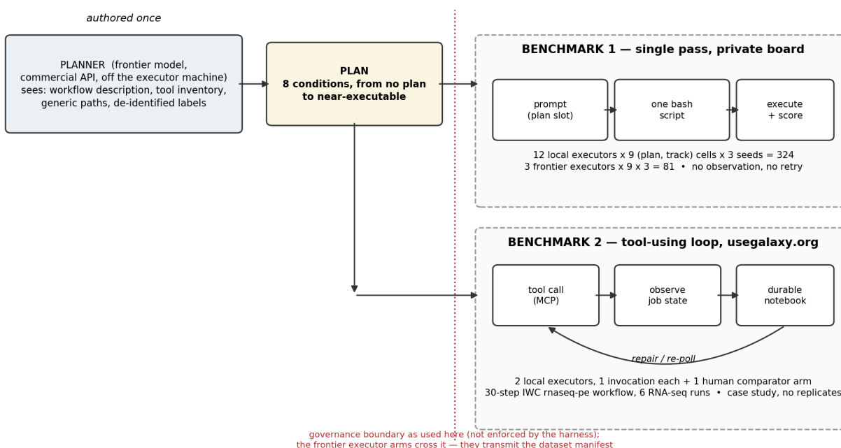
Figure 1. Study design. A plan is authored once, off the executor machine, by a frontier model in the planner role. Benchmark 1 executes that plan in a single pass: one prompt in, one bash script out, executed and scored with no observation step. Benchmark 2 executes it in a tool-using loop against the public usegalaxy.org server, with observation, durable state and repair. The dotted line marks the data-governance boundary as it was
