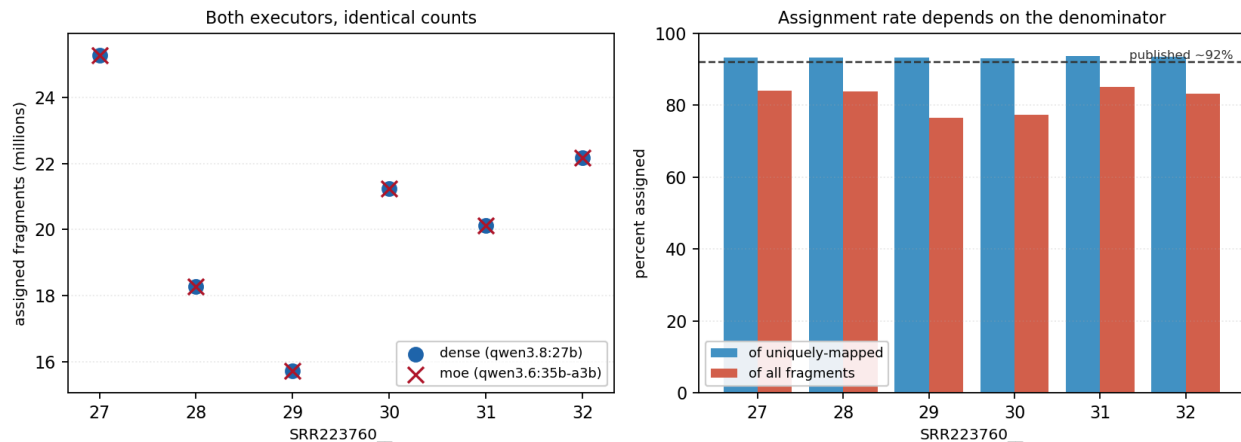
Figure 5. Per-sample featureCounts results for the benchmark-2 case study. Left: assigned fragments per run; the dense (qwen3.8:27b) and mixture-of-experts (qwen3.6:35b-a3b) arms are exactly superimposed. Right: assignment rate against two denominators — uniquely mapped fragments and all fragments — with the published ~92% benchmark marked. The gap between the two denominators is multi-mapping, a property of the data rather than of the executor.
