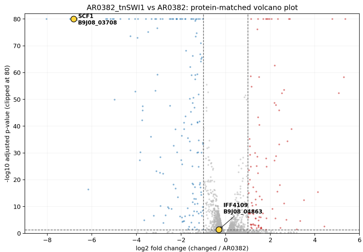
Figure 1. Volcano plot for AR0382_tnSWI1 vs AR0382. Yellow points highlight protein-matched SCF1 (B9J08_03708) and IFF4109 (B9J08_04863). SCF1 is among the strongest downregulated genes.
