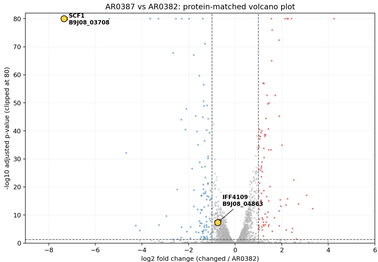
Figure 2. Volcano plot for AR0387 vs AR0382. Protein-matched SCF1 is again strongly downregulated, although this secondary contrast should be interpreted with more caution because AR0387_B had lower mapping metrics.
