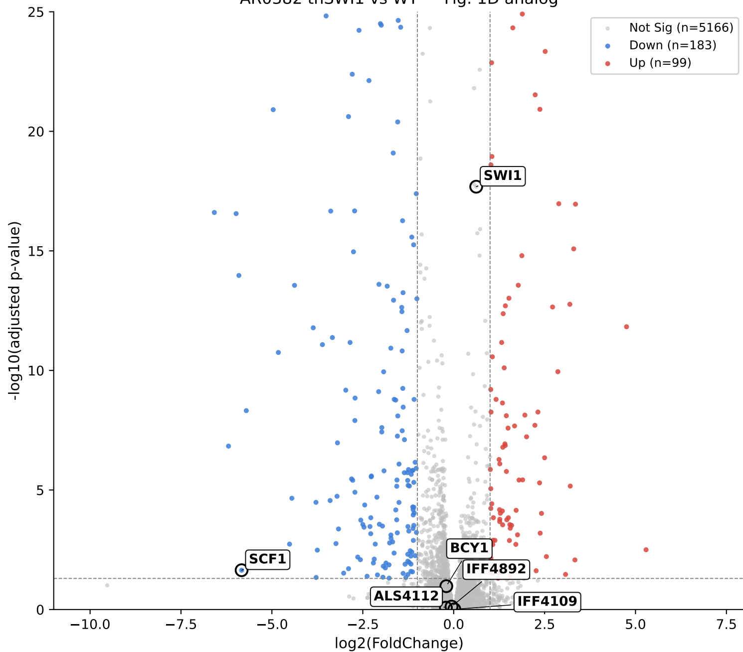
AR0382 tnSWI1 vs WT — Fig. 1D analog
