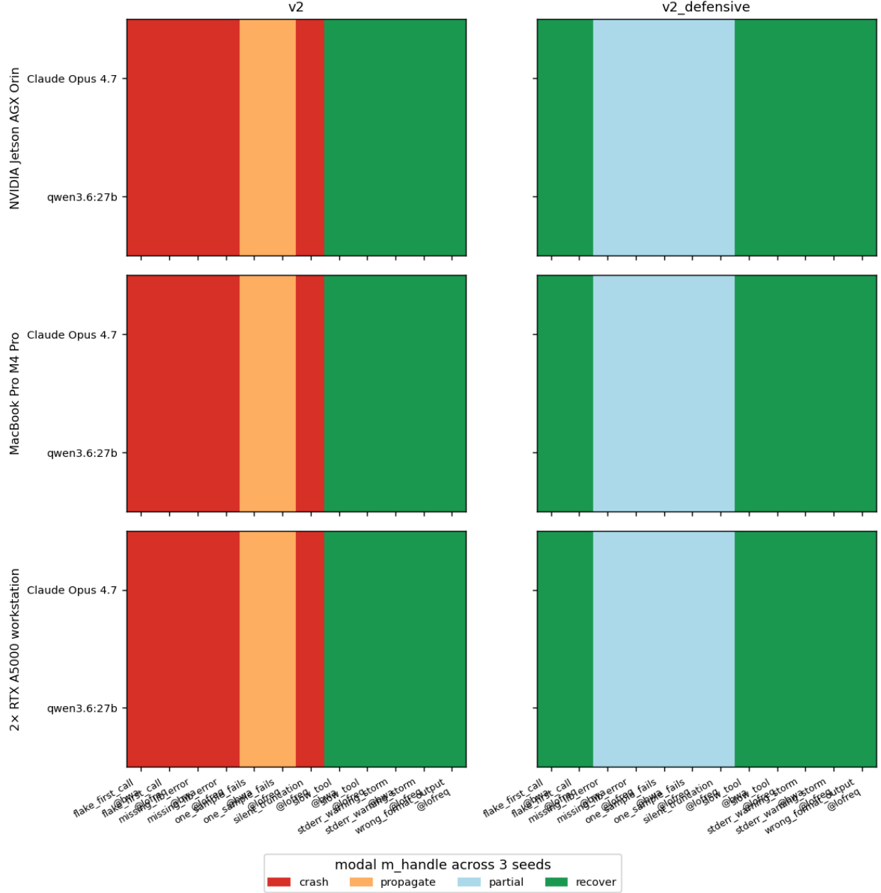
Figure 2: Figure 3. Per-cell error-handling outcome (recover / partial / propagate / crash) for claude-opus-4-7 and qwen3.6:27b across the 12-cell PATH-shim error matrix on three hardware platforms. Left column = v2 baseline plan; right column = v2_defensive plan. Rows within each panel are the two models. Cells are color-coded by the modal m_handle outcome across three seeds.
