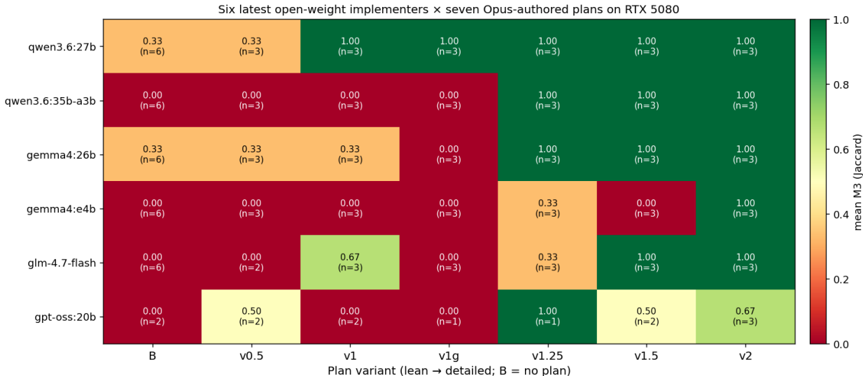
Figure 1: Figure 2. Mean M3 across three seeds for six open-weight implementers \times seven Opus-authored plan variants on the RTX 5080. Columns are ordered by plan detail (left = no plan, right = most detailed). Anthropic API plan-author rows are not shown here because Anthropic models execute on Anthropic’s own hardware; they appear in the cross-platform error-injection panel below.
