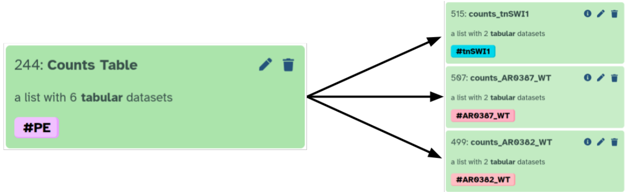
Figure 1: CCA splits collection containing counts into three collections corresponding to three different strains (conditions).
