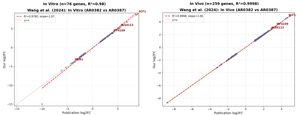
Figure 3: Validation of Wang et al. DESeq2 results using official NCBI gene ID mapping. Left: In
