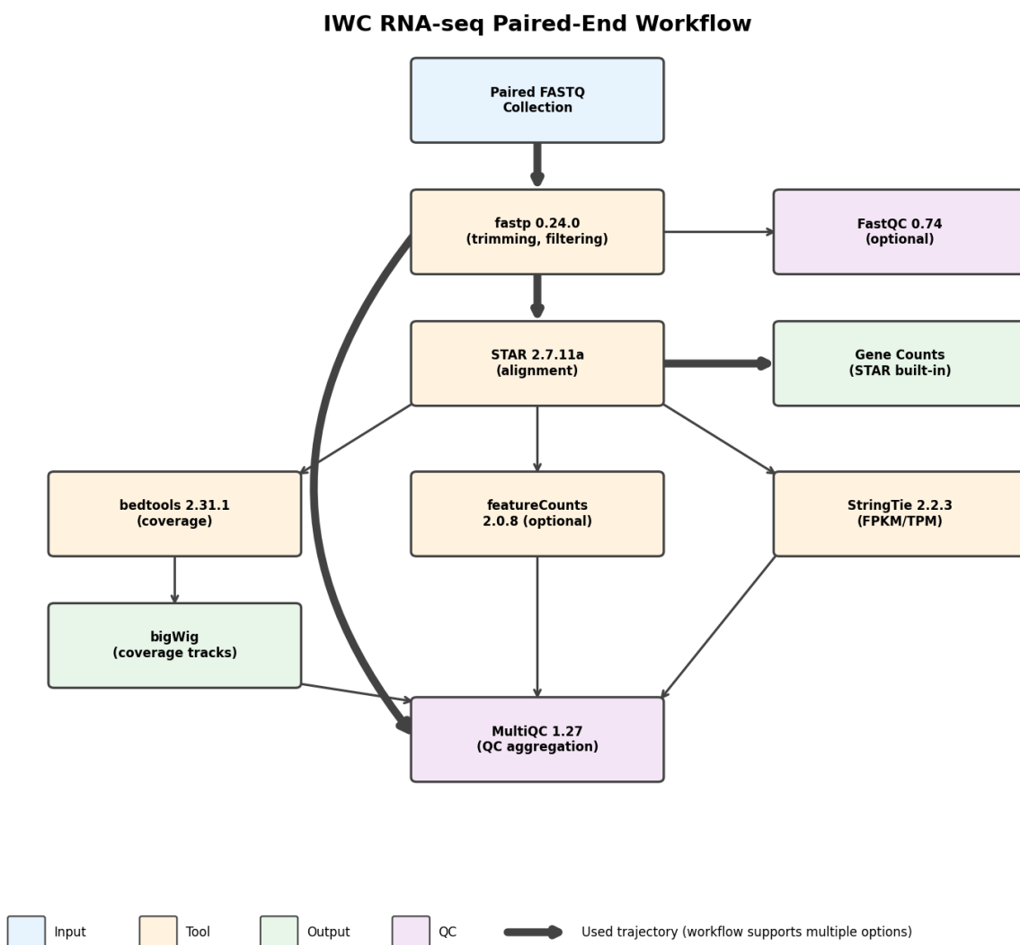
Figure 4: IWC paired-end RNA-seq workflow. The pipeline processes FASTQ files through quality filtering ( fastp ), alignment ( STAR ), and quantification, with optional coverage track generation and QC aggregation via MultiQC .
