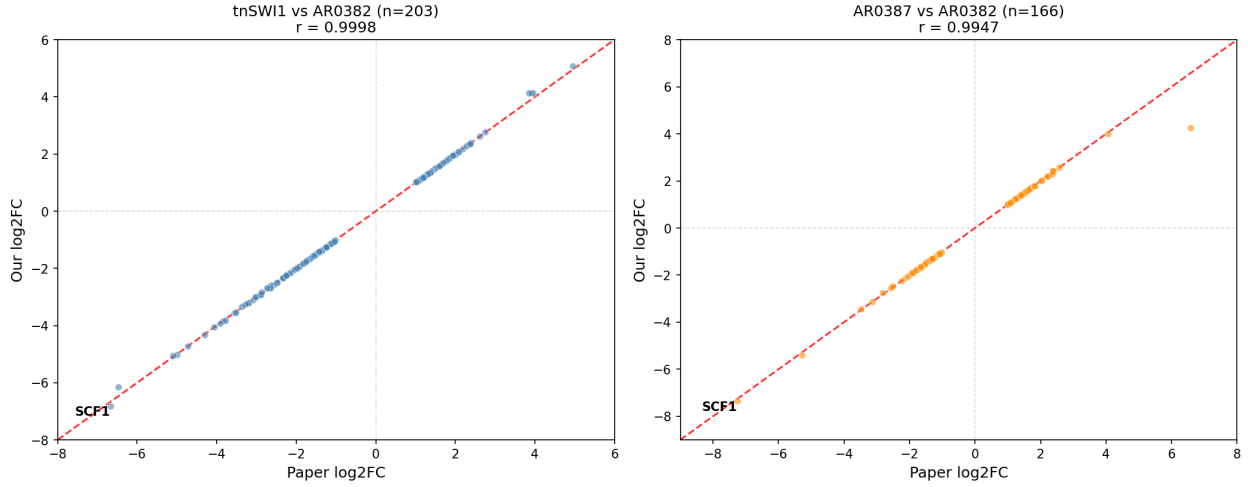
Figure 1: Validation of Santana et al. DESeq2 results. Left: tnSWI1 vs AR0382 comparison (Fig 1D). Right: AR0387 vs AR0382 comparison (Fig S5A). Red dashed line indicates perfect correlation ( y=x ).
