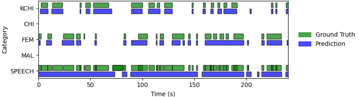
Figure 3. VTC_{cl} Predictions compared to Ground Truth Annotations
