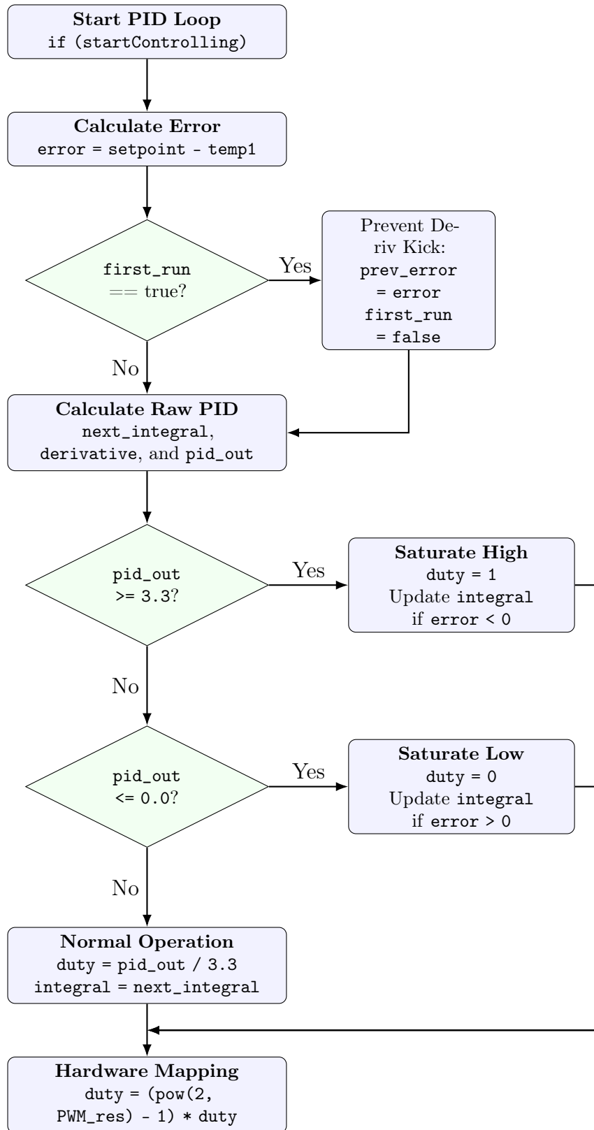
Figure 19: Software execution flow of the discrete PID algorithm, highlighting first-run derivative protection and integral anti-windup logic.
