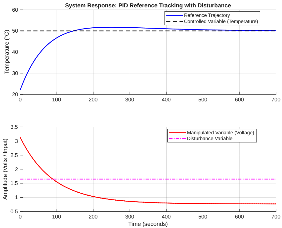
Figure 16: PID reference tracking control with disturbance
