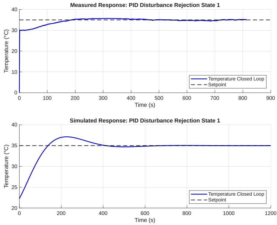
Figure 24: Measured Results for PID disturbance rejection tracking for state 1
