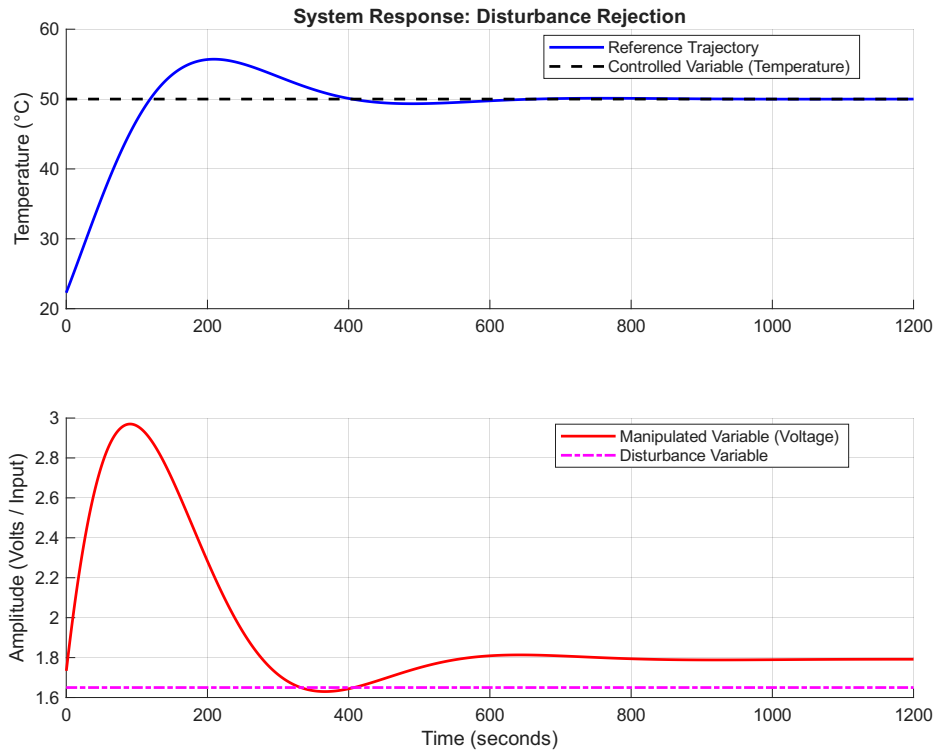
(b) Closed-loop response (50% PWM Disturbance).
