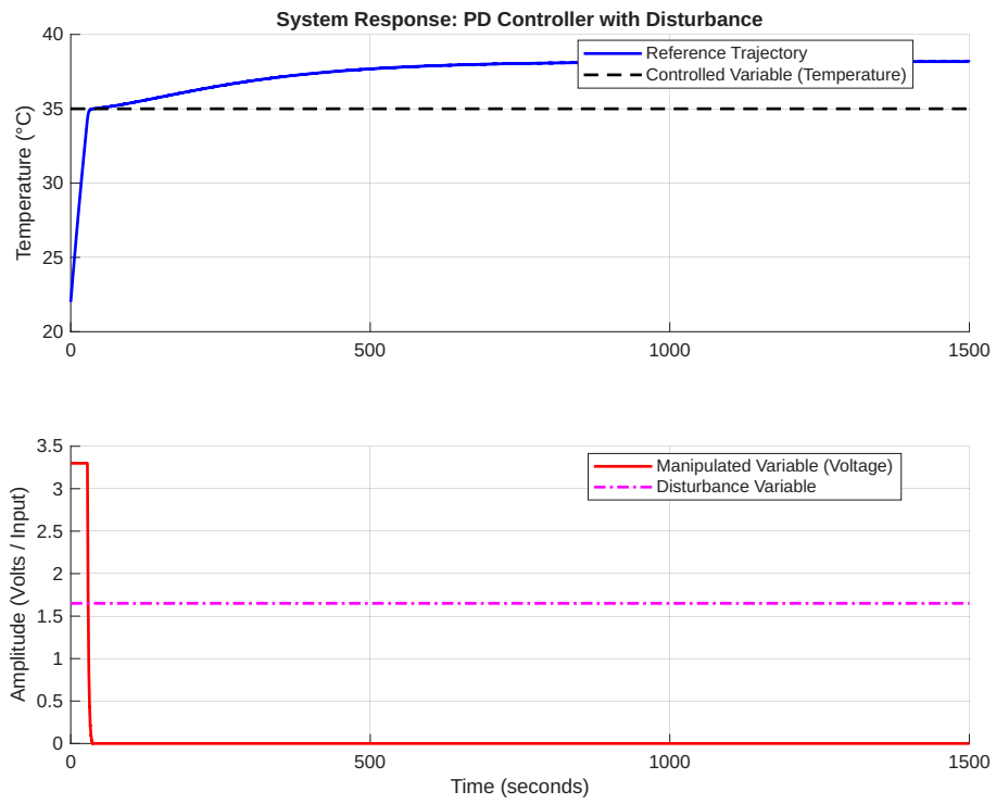
Figure 13: PD Control with disturbance
