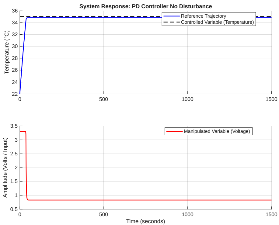
Figure 12: PD Control with no disturbance
