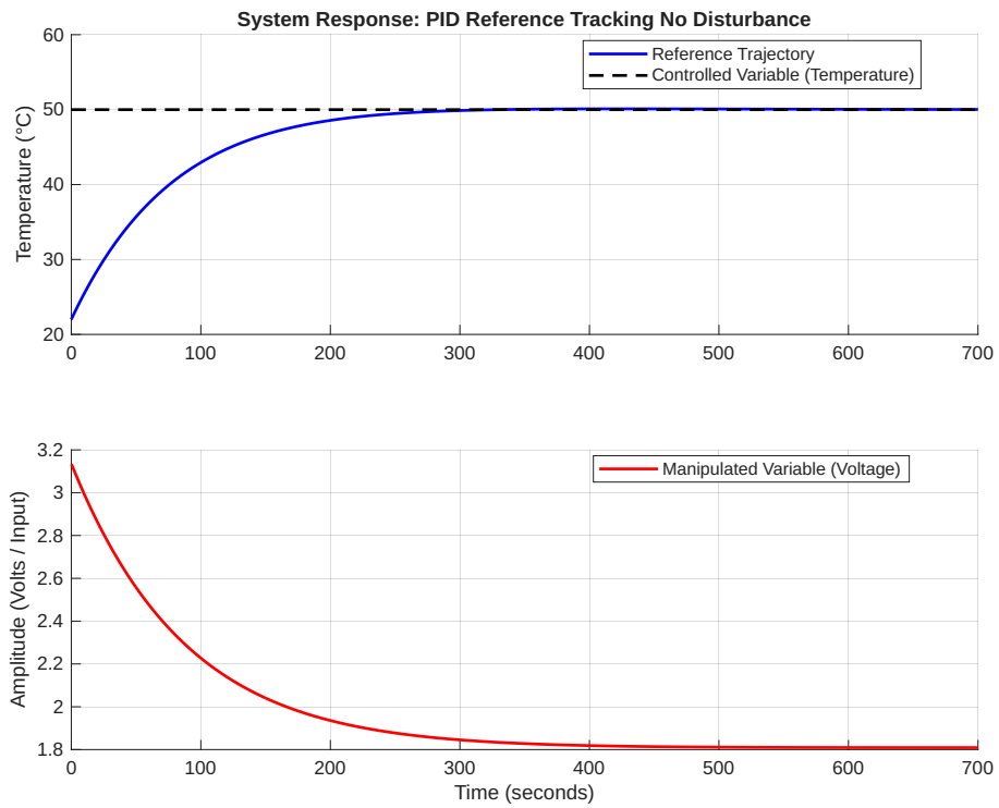
Figure 15: PID reference tracking control with no disturbance
