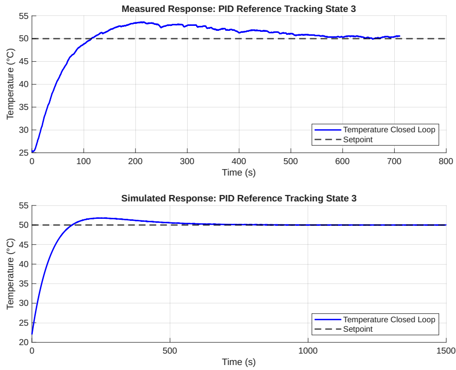
Figure 22: Measured Results for PID reference tracking for state 3
