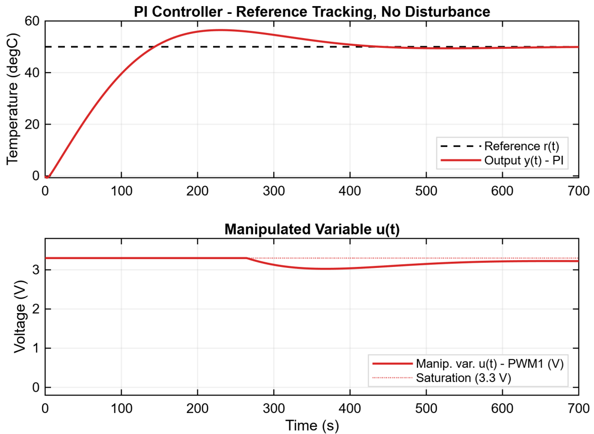
Figure 8: Closed-loop response of the PI controller with no disturbance. Top: reference trajectory and controlled variable (temperature). Bottom: manipulated variable (PWM1 voltage).
