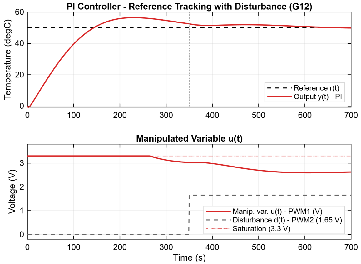
Figure 9: Closed-loop response of the PI controller with disturbance via G_{12} . Top: reference and controlled variable. Bottom: manipulated variable (PWM1) and disturbance input (PWM2).
