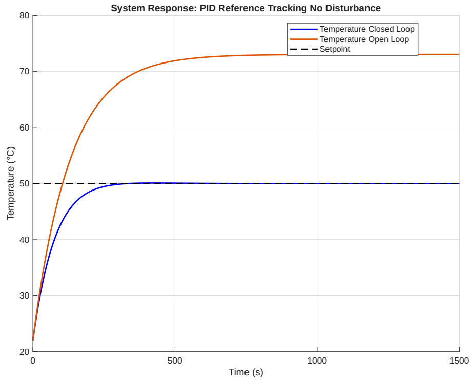
Figure 14: Comparing the closed loop step response for the PID reference tracking controller to the open loop step response
