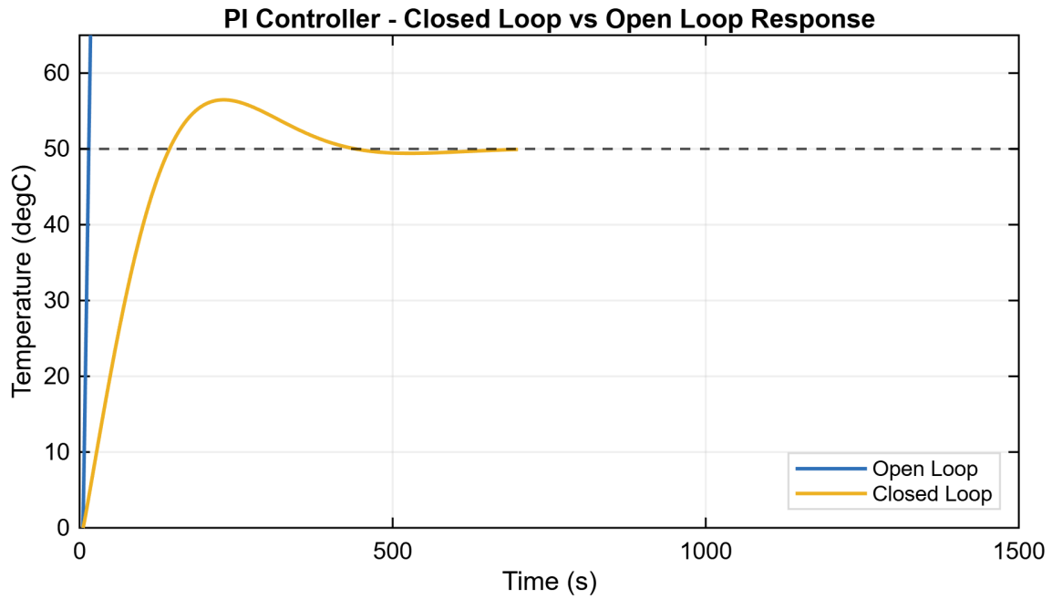
Figure 7: Closed-loop vs open-loop step response of the PI controller. The integral term eliminates the steady-state error present in the P controller, with the closed-loop output converging exactly to the 50 °C reference.
