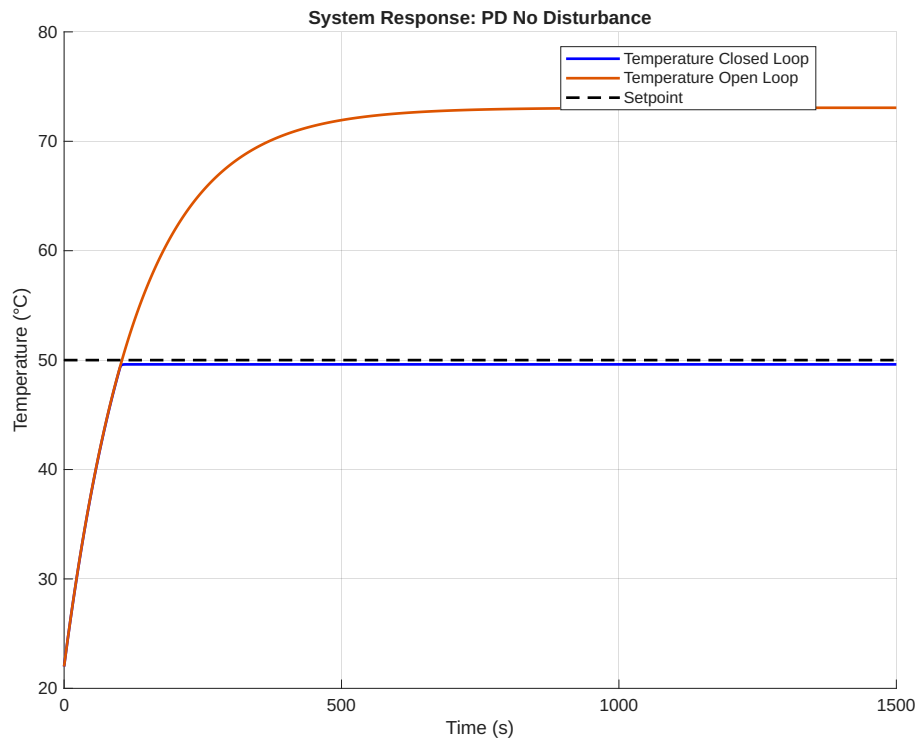
Figure 11: Comparing the closed loop PD controller step response to the open loop step response.
