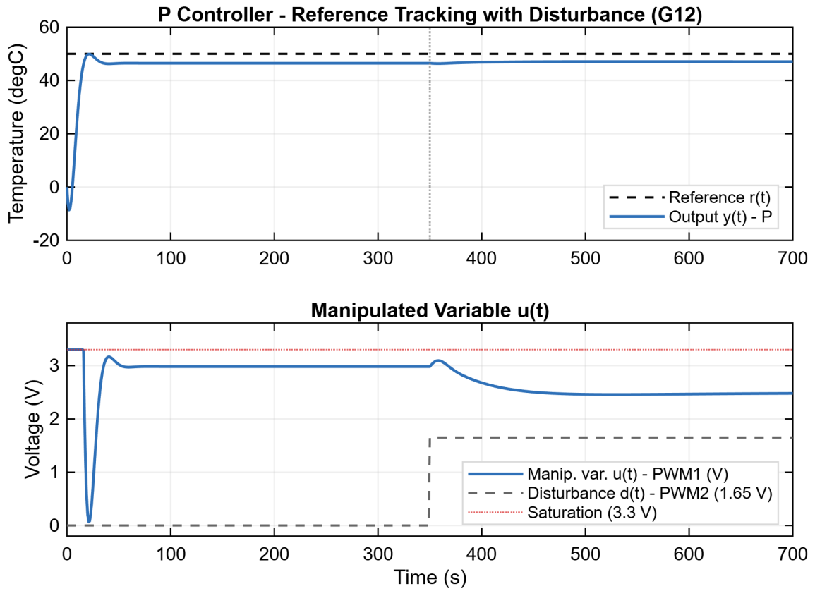
Figure 6: Closed-loop response of the P controller with disturbance via G_{12} . Top: reference and controlled variable. Bottom: manipulated variable (PWM1) and disturbance input (PWM2).
