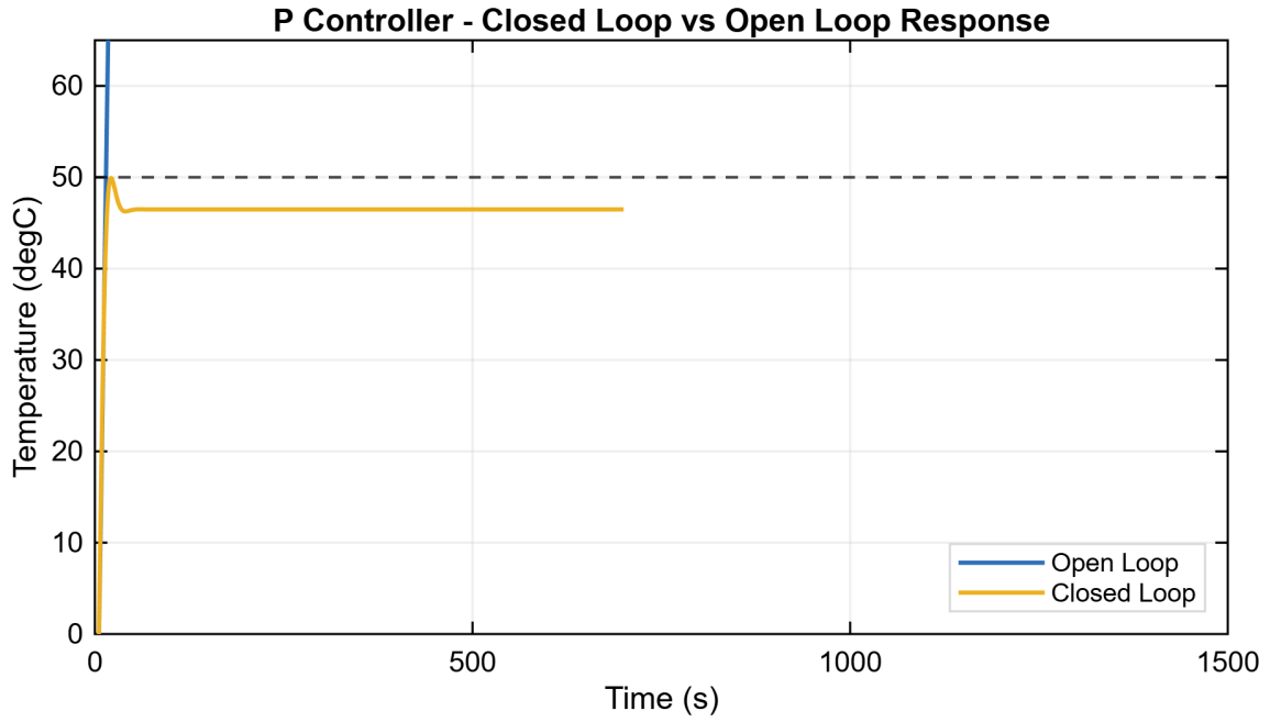
Figure 4: Closed-loop vs open-loop step response of the P controller. The closed-loop response reaches the reference significantly faster but exhibits overshoot and a steady-state error due to the absence of an integral term.
