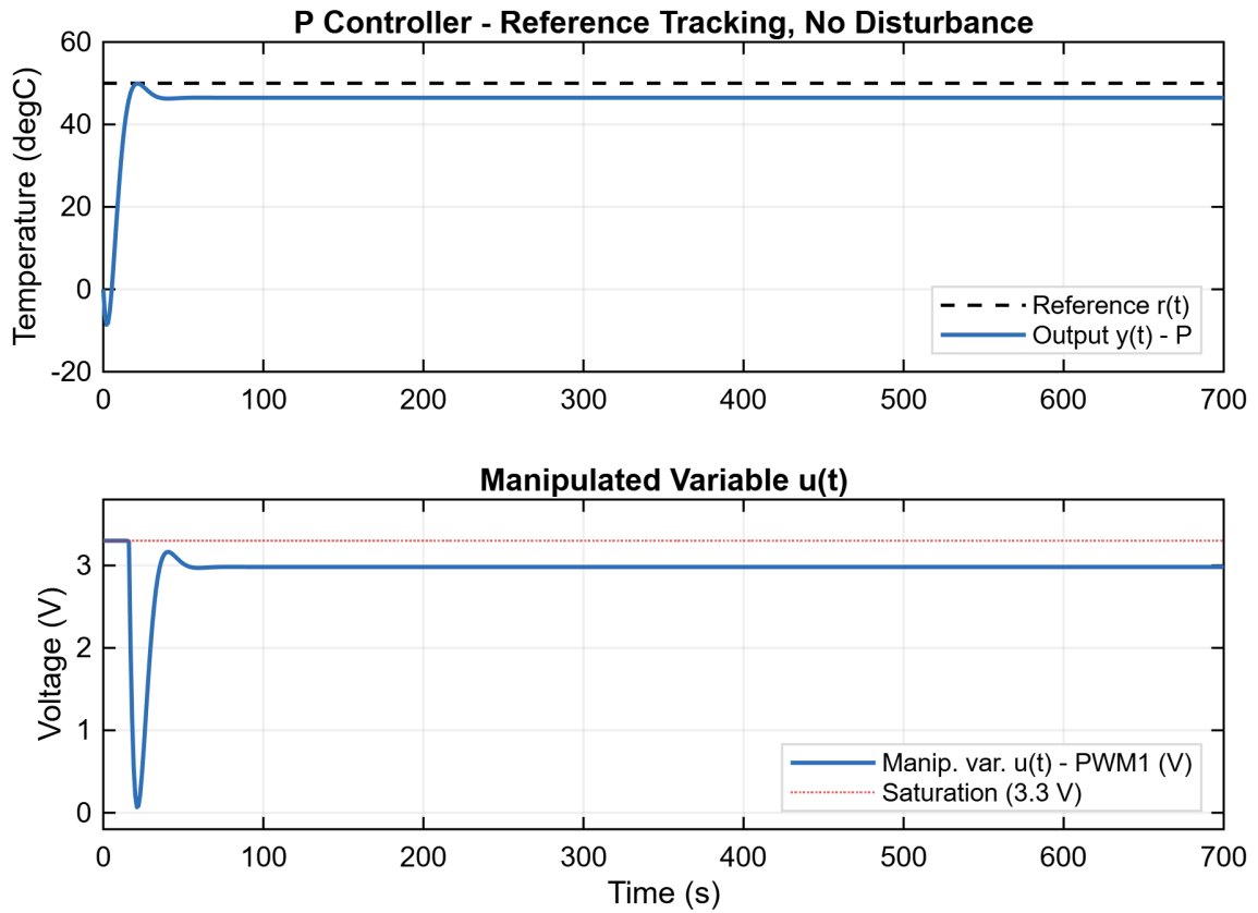
Figure 5: Closed-loop response of the P controller with no disturbance. Top: reference trajectory and controlled variable (temperature). Bottom: manipulated variable (PWM1 voltage).
