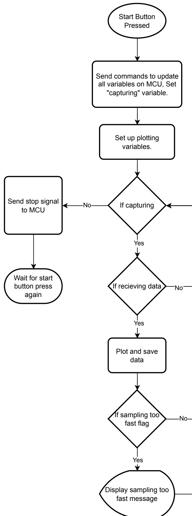
Figure 2: Flow Diagram of Matlab Code.
