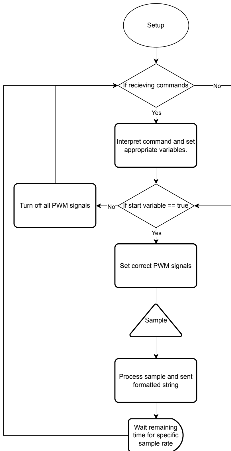
Figure 1: Flow Diagram of MCU Code.
