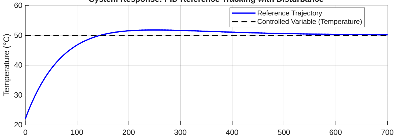
System Response: PID Reference Tracking with Disturbance
