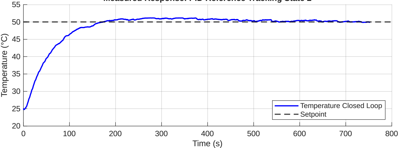
Measured Response: PID Reference Tracking State 2
