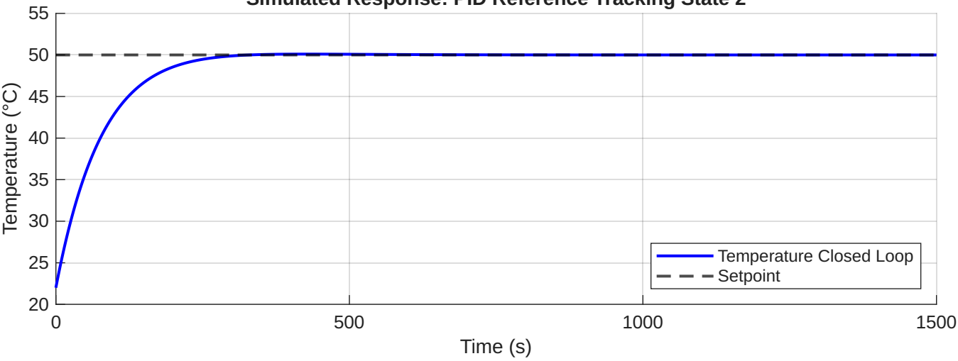
Simulated Response: PID Reference Tracking State 2
