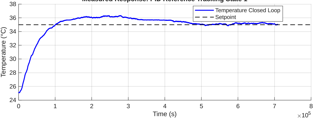
Measured Response: PID Reference Tracking State 1
