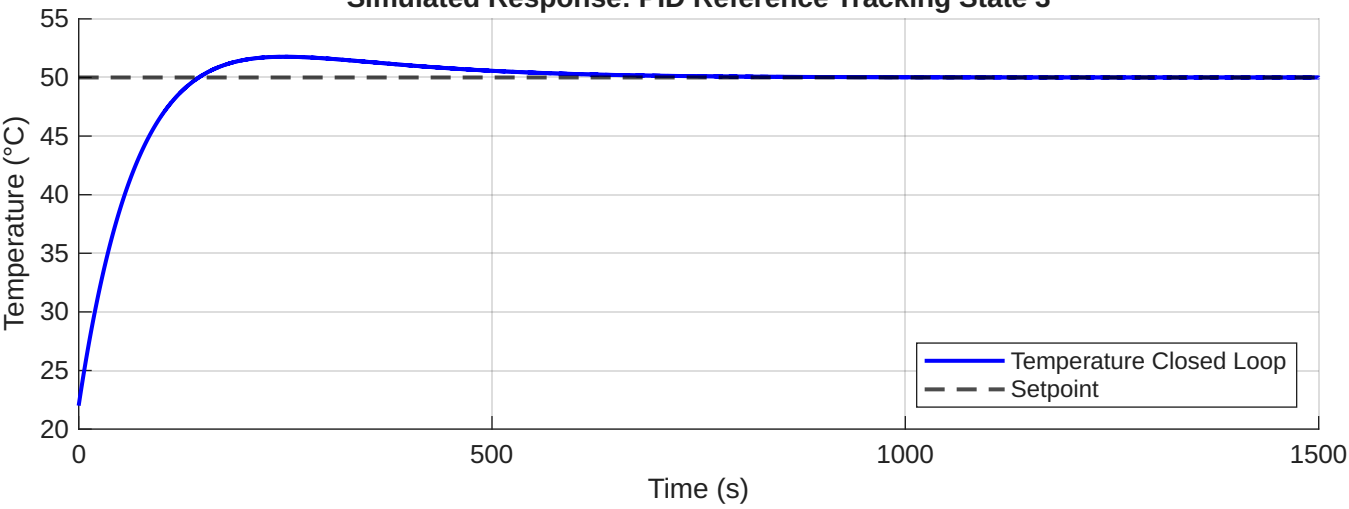
Simulated Response: PID Reference Tracking State 3
