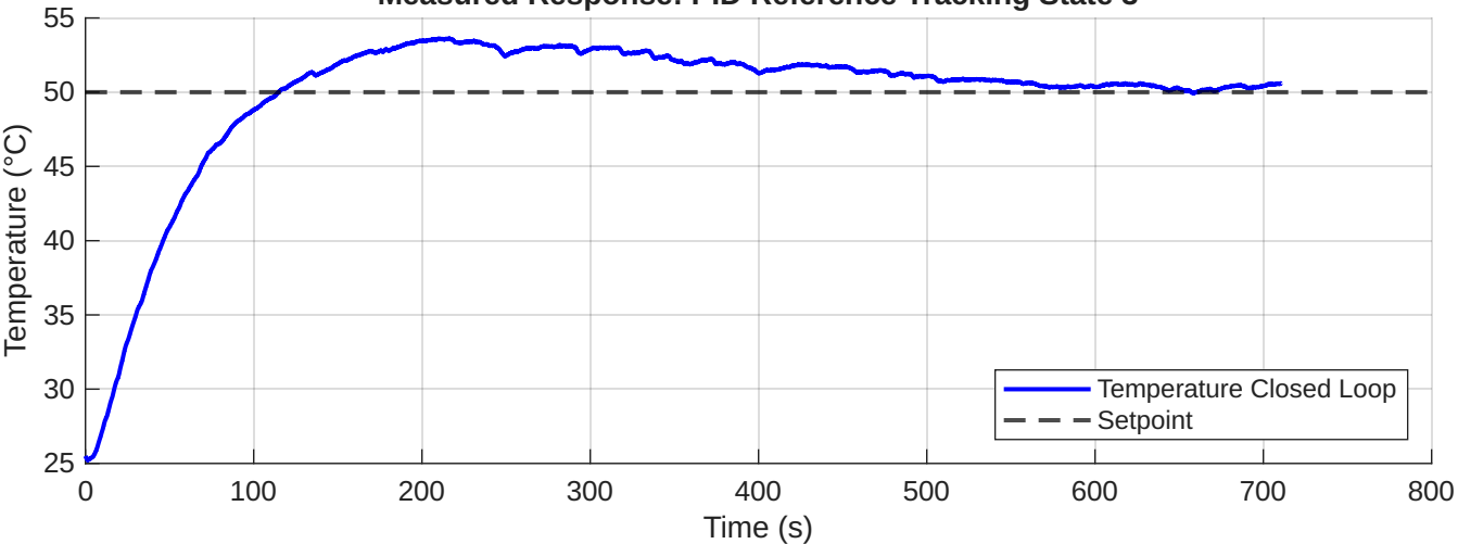
Measured Response: PID Reference Tracking State 3
