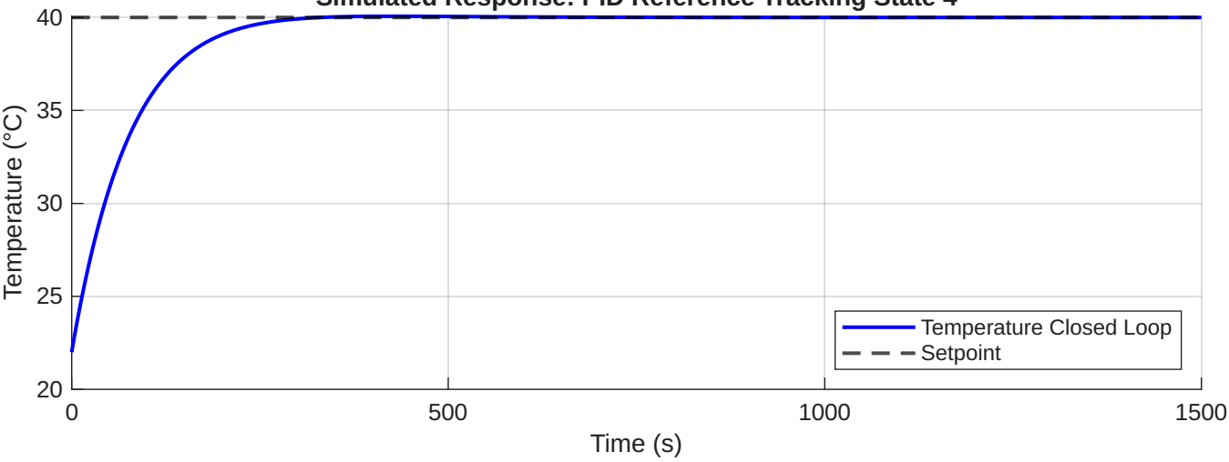
Simulated Response: PID Reference Tracking State 4
