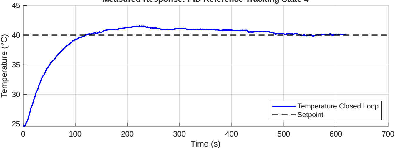
Measured Response: PID Reference Tracking State 4
