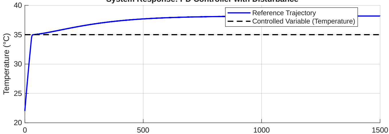
System Response: PD Controller with Disturbance
