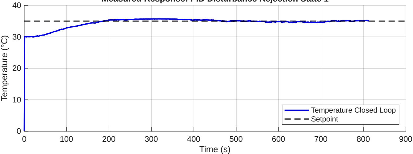
Measured Response: PID Disturbance Rejection State 1
