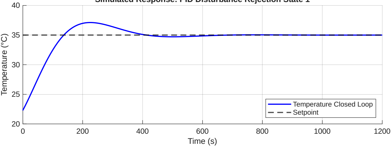
Simulated Response: PID Disturbance Rejection State 1
