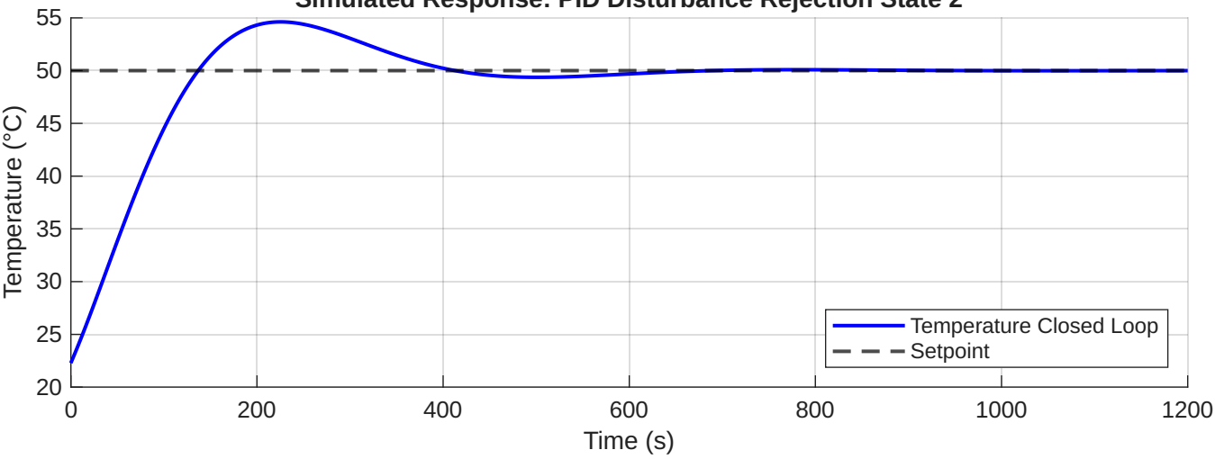
Simulated Response: PID Disturbance Rejection State 2
