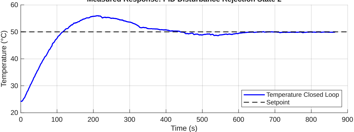
Measured Response: PID Disturbance Rejection State 2
