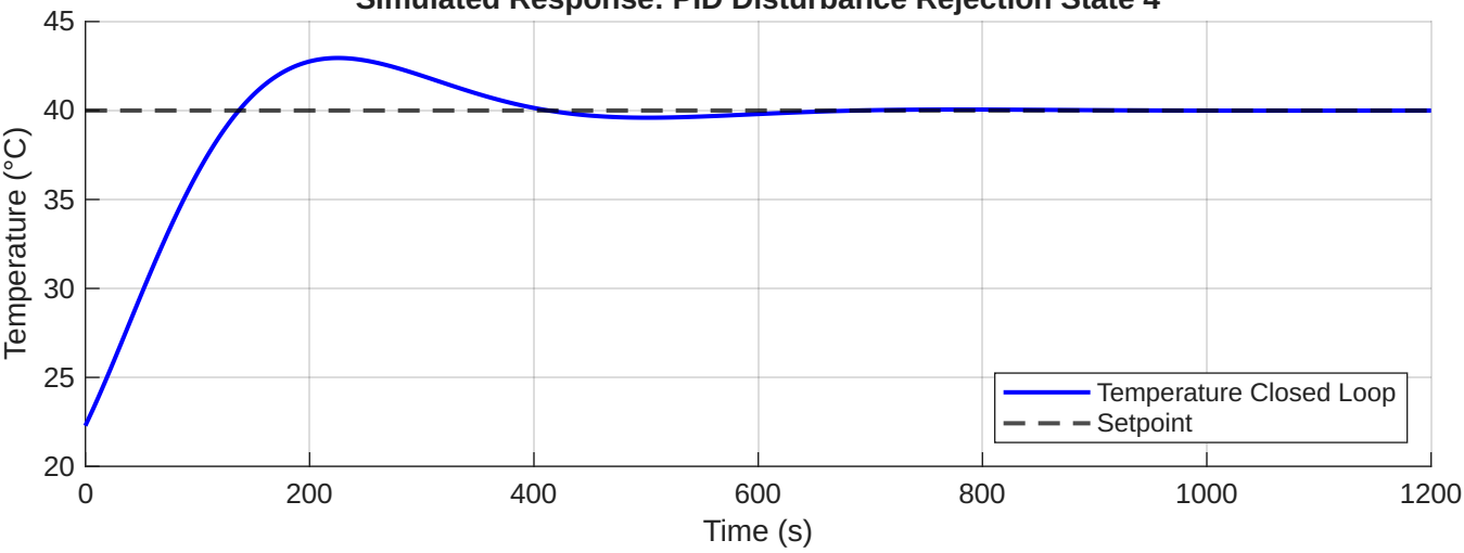
Simulated Response: PID Disturbance Rejection State 4
