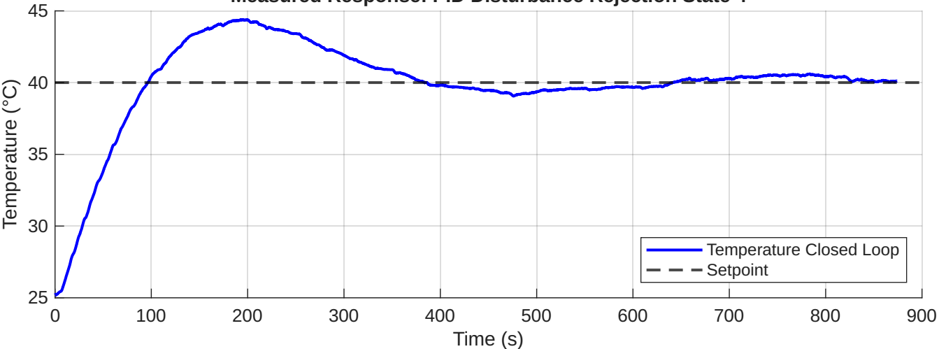
Measured Response: PID Disturbance Rejection State 4
