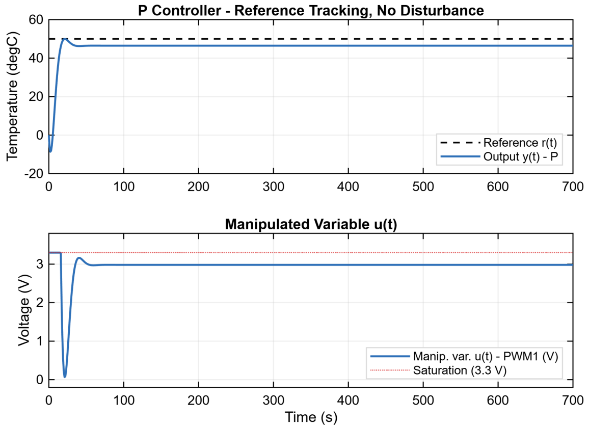
Figure 2: Closed-loop response of the P controller with no disturbance. Top: reference trajectory and controlled variable (temperature). Bottom: manipulated variable (PWM1 voltage).
