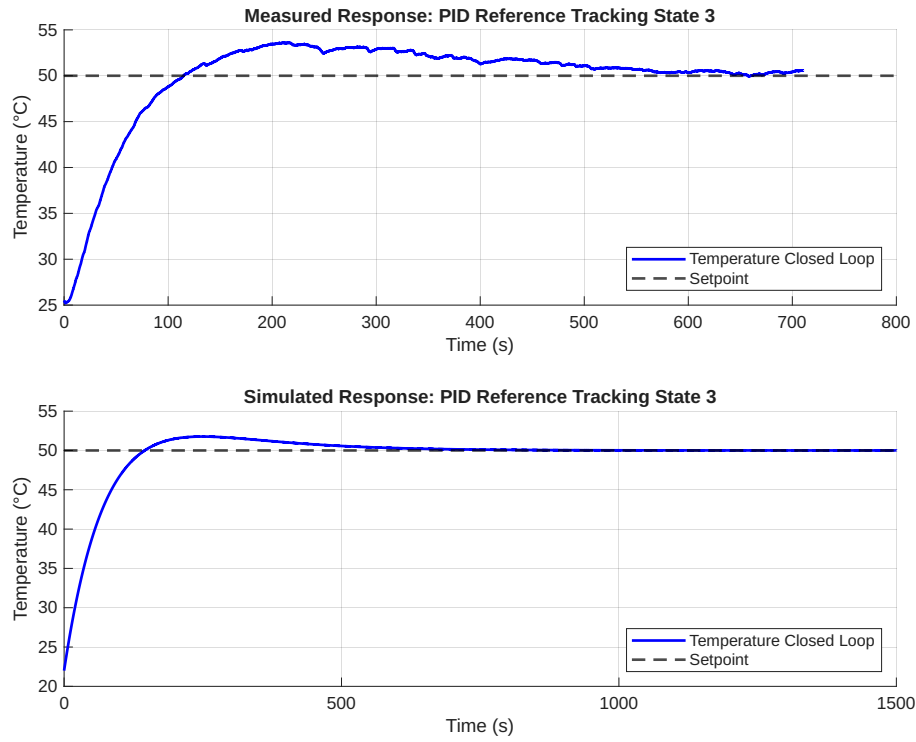
Figure 17: Measured Results for PID reference tracking for state 3
