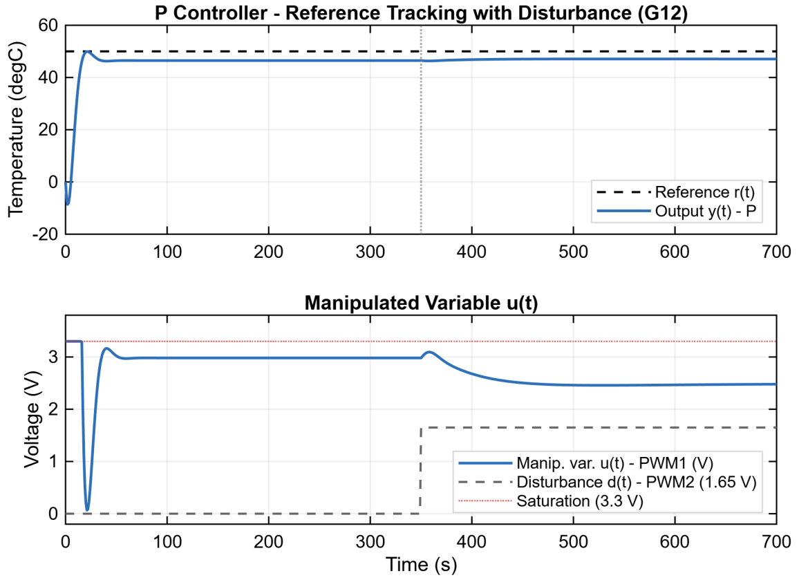
Figure 3: Closed-loop response of the P controller with disturbance via G_{12} . Top: reference and controlled variable. Bottom: manipulated variable (PWM1) and disturbance input (PWM2).
