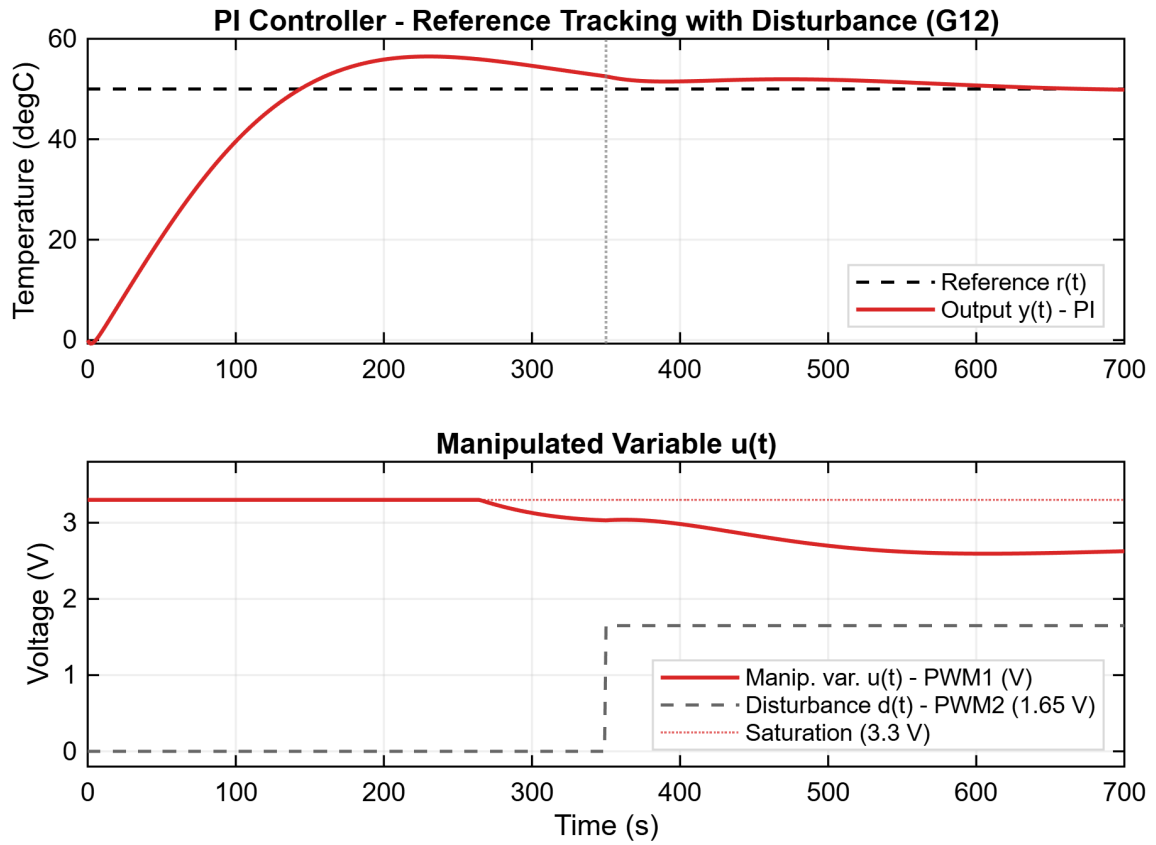
Figure 5: Closed-loop response of the PI controller with disturbance via G_{12} . Top: reference and controlled variable. Bottom: manipulated variable (PWM1) and disturbance input (PWM2).
