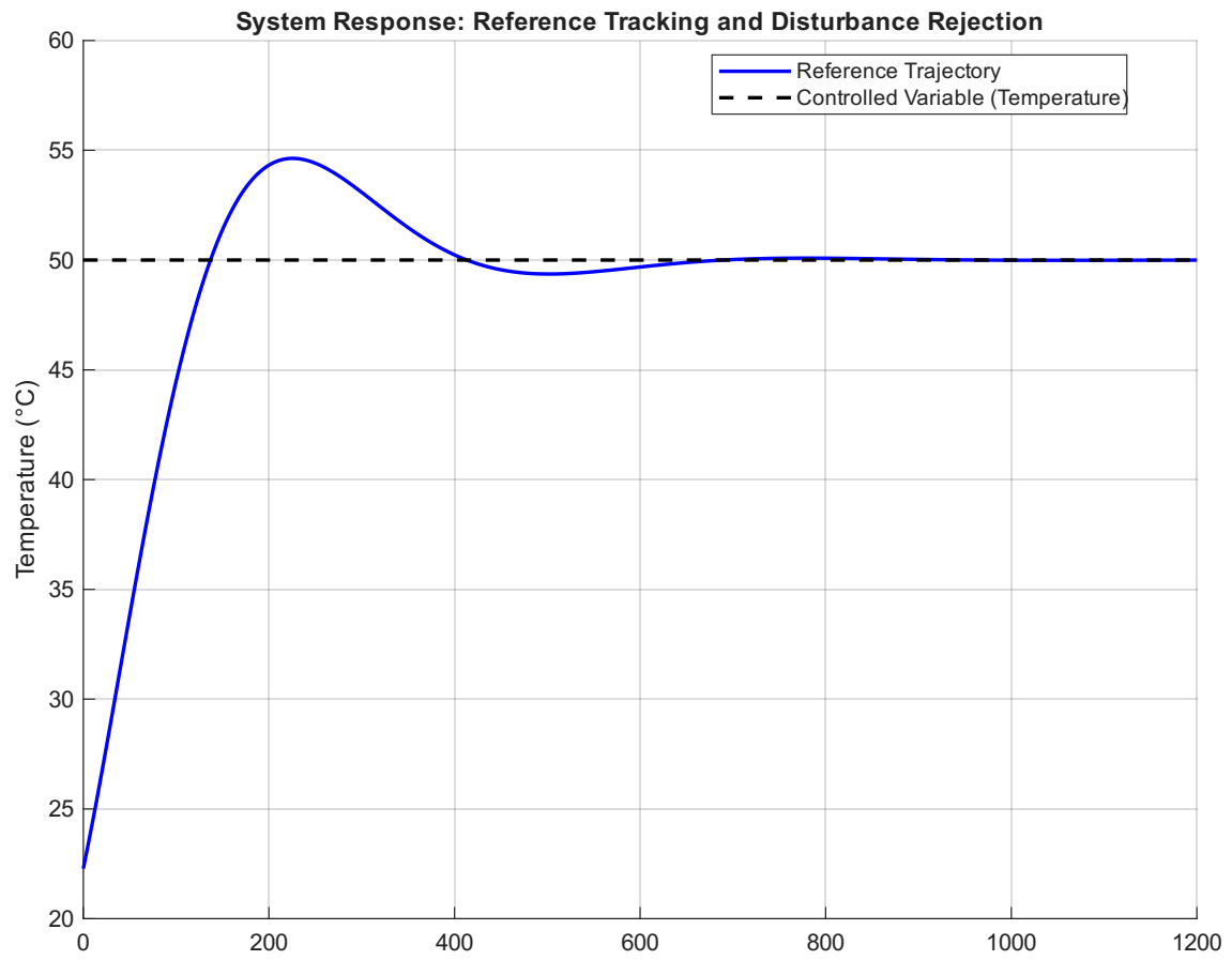
Figure 12: Closed Loop response of PID Disturbance Rejection Controller
