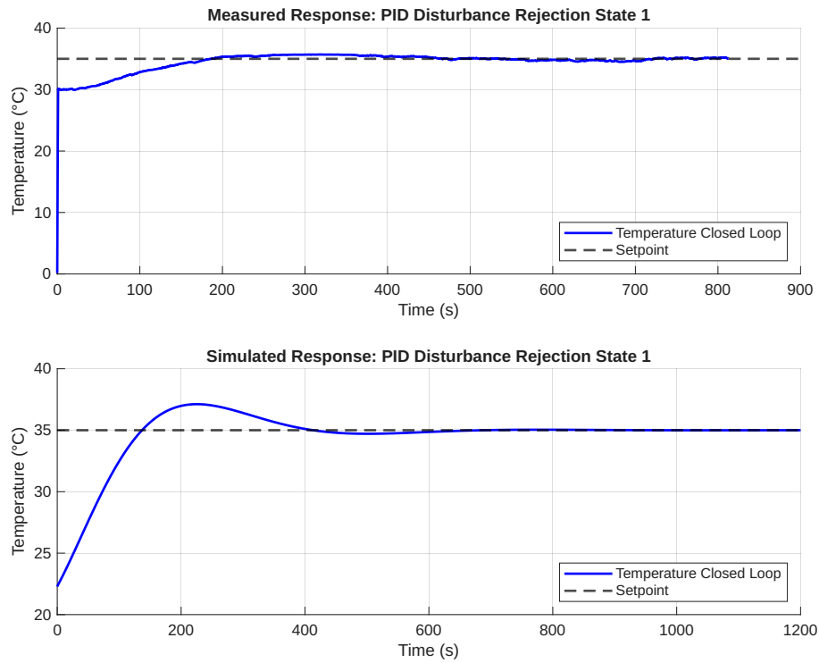
Figure 19: Measured Results for PID disturbance rejection tracking for state 1
