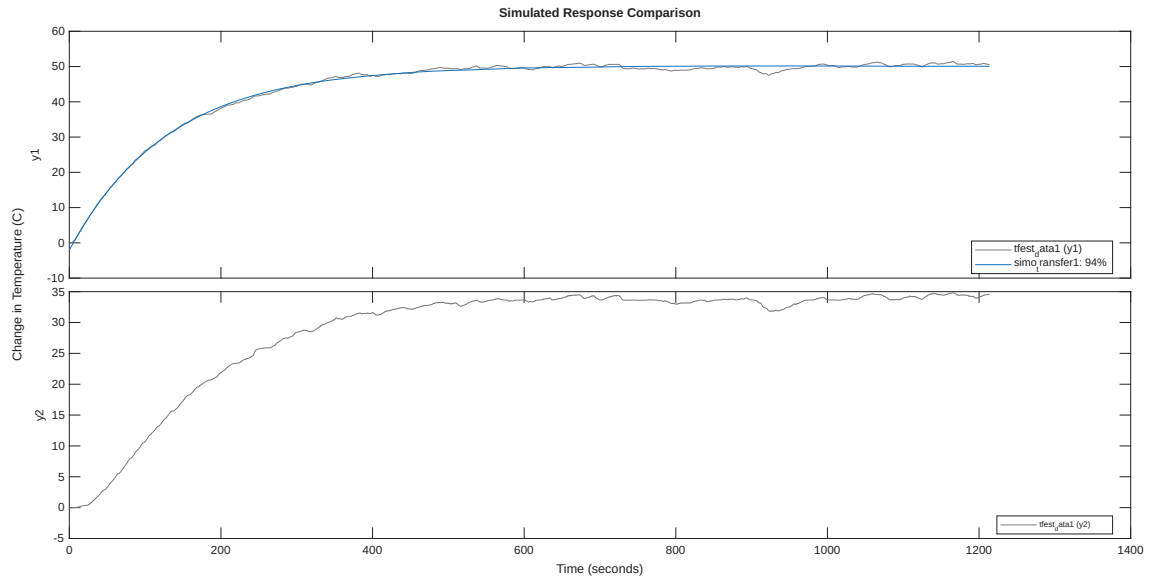
Figure 1: Accuracy comparison of G_{11} 's transfer function
