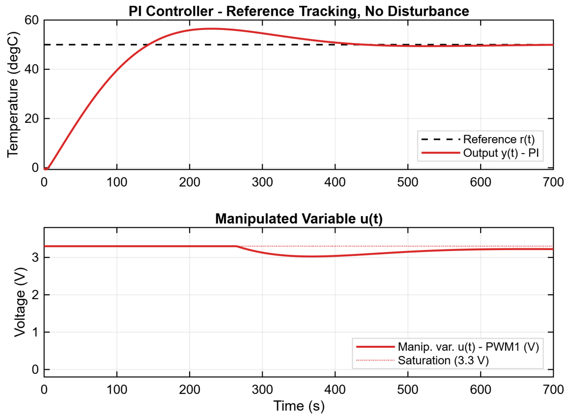
Figure 4: Closed-loop response of the PI controller with no disturbance. Top: reference trajectory and controlled variable (temperature). Bottom: manipulated variable (PWM1 voltage).
