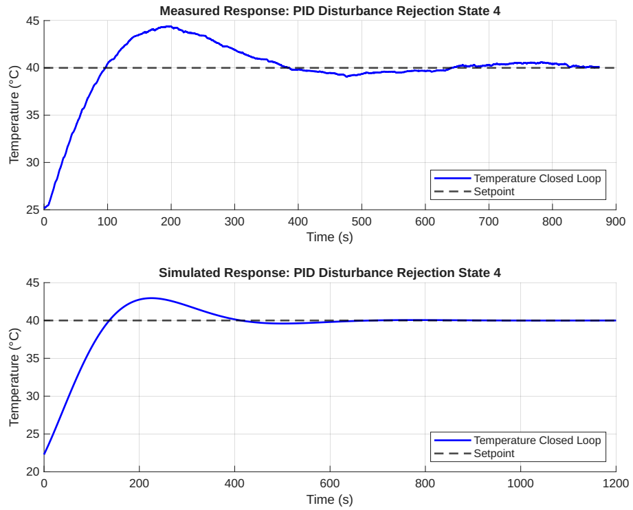
Figure 22: Measured Results for PID disturbance rejection tracking for state 4
