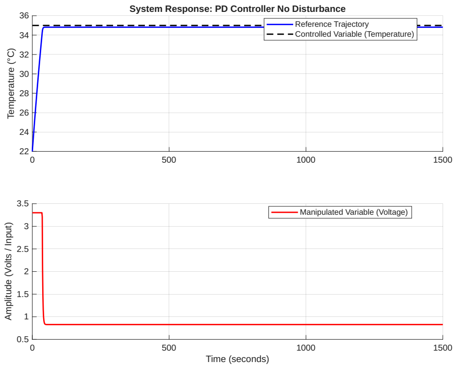
Figure 7: PD Control with no disturbance
