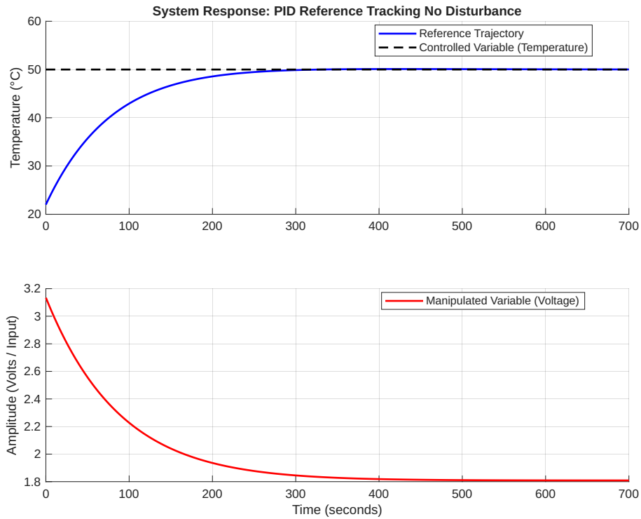
Figure 9: PID reference tracking control with no disturbance
