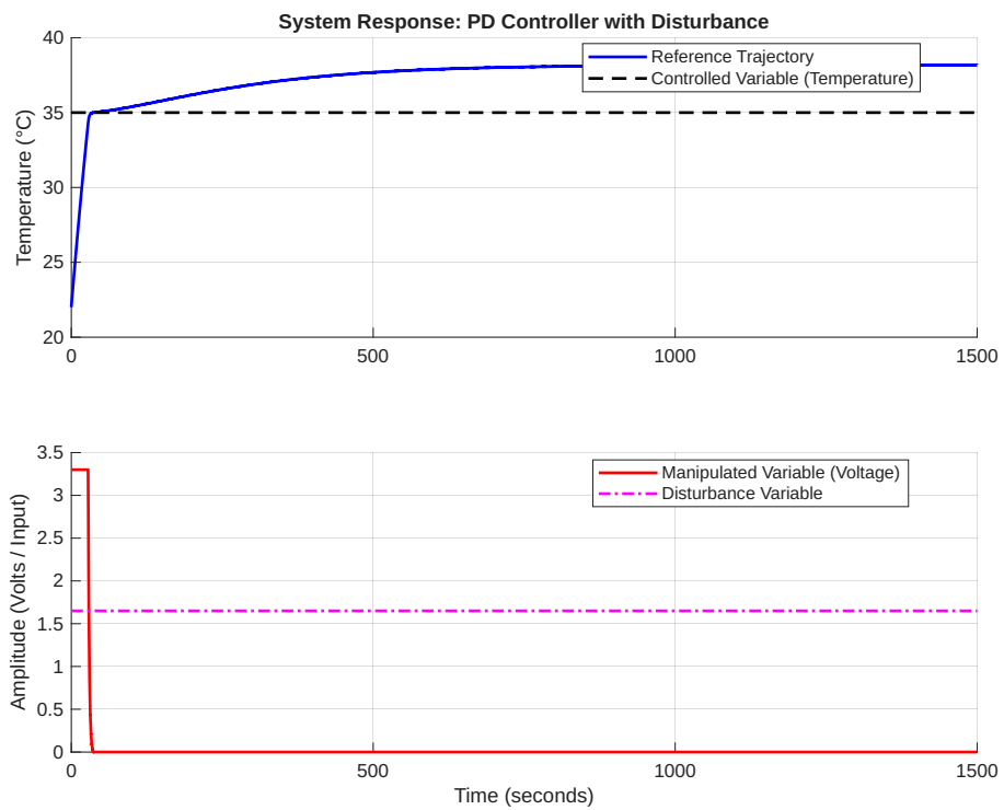
Figure 8: PD Control with disturbance
