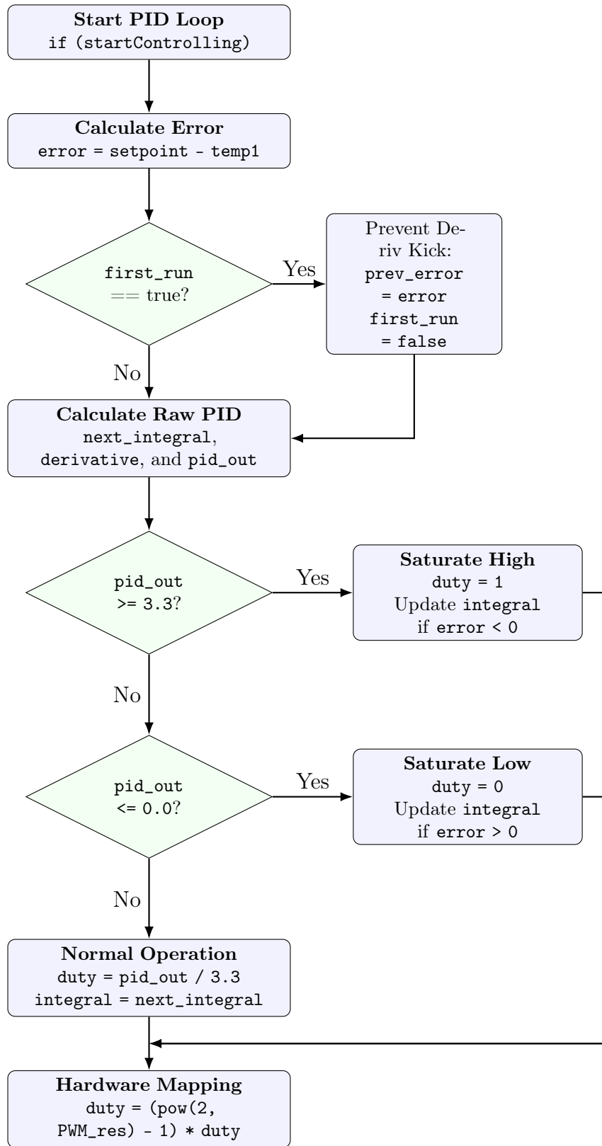
Figure 14: Software execution flow of the discrete PID algorithm, highlighting first-run derivative protection and integral anti-windup logic.
