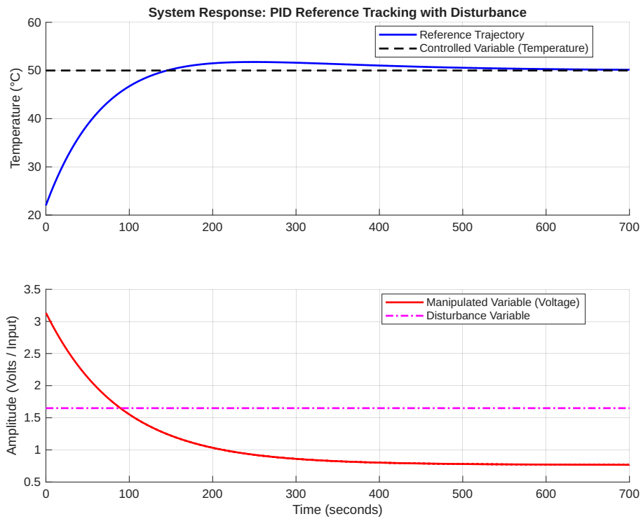
Figure 10: PID reference tracking control with disturbance
