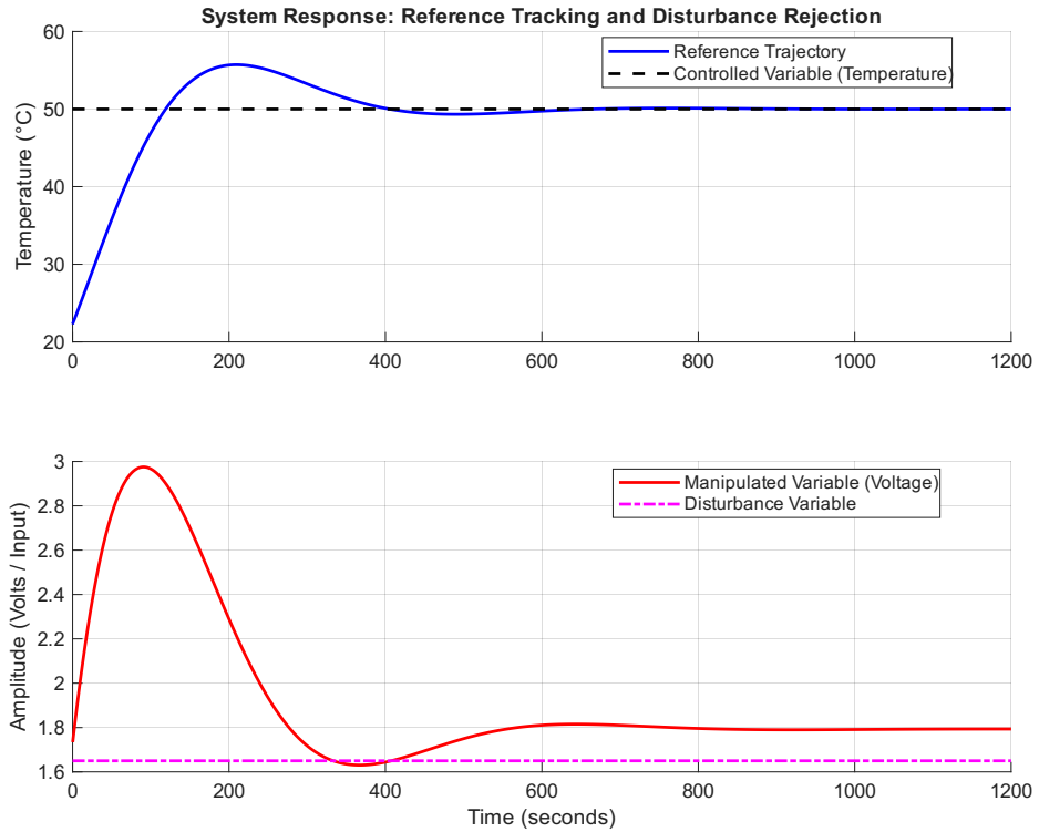
(b) Closed-loop response (50% PWM Disturbance).
