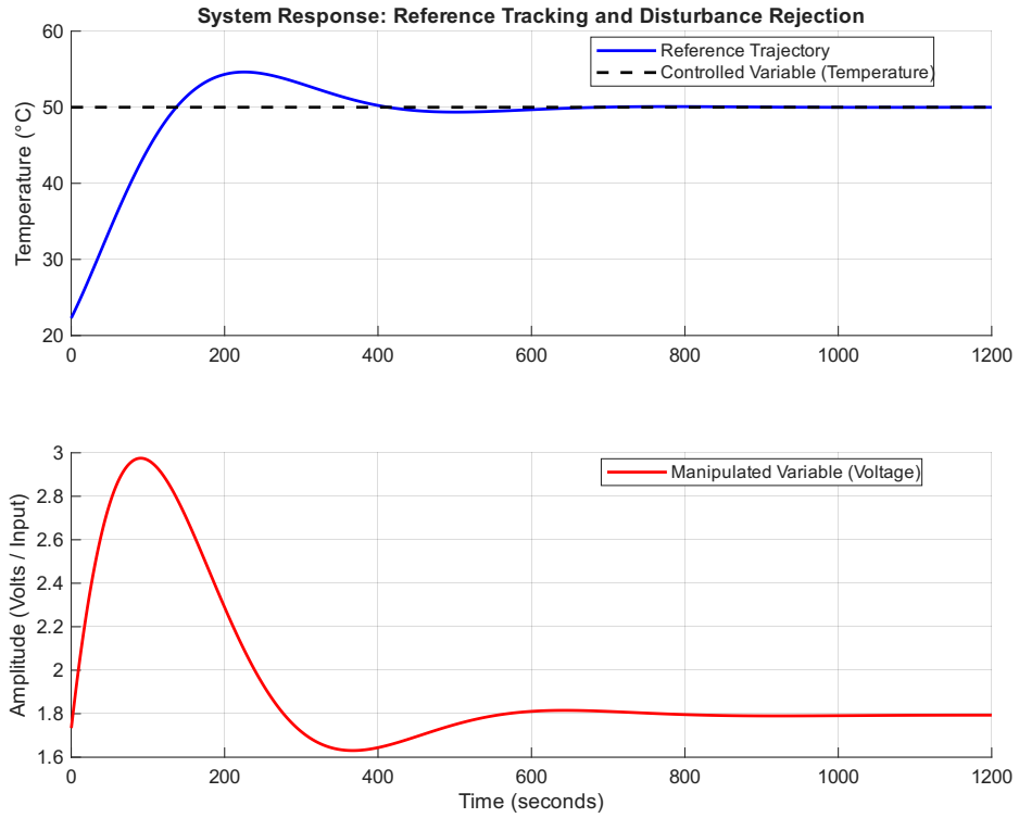
(a) Closed-loop response (No Disturbance).
